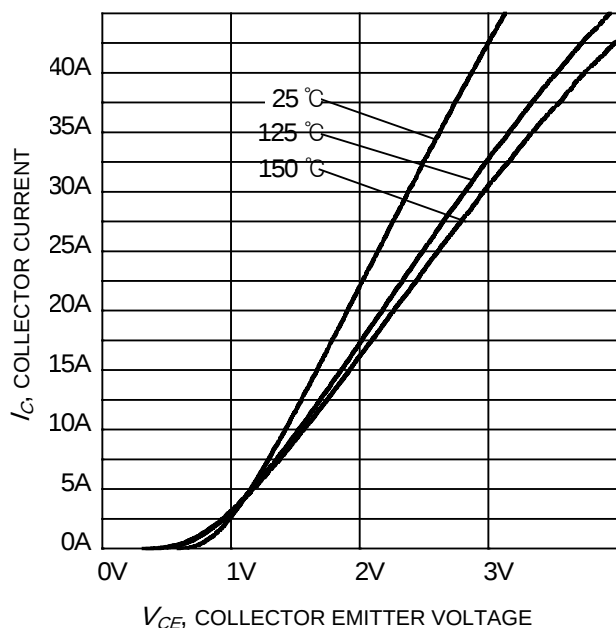
Figure 4. Typical IGBT output characteristic ( V_{DD} = 15\text{V} )
