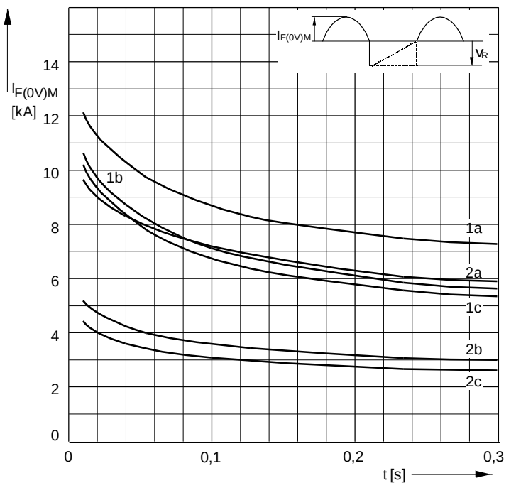
Bild / Fig. 4 Grenzstrom / Maximum overload forward current I_{F(0V)M} = f(t) 1 - I_{FAV(vor)} = 0\text{ A} ; t_{j} = t_c = 25\text{ °C} 2 - I_{FAV(vor)} = 400\text{ A} ; t_c = 130\text{ °C} ; t_{j} = 180\text{ °C} a - V_R \leq 50\text{ V} b - V_R = 0,5 V_{RRM} c - V_R = 0,8 V_{RRM}
