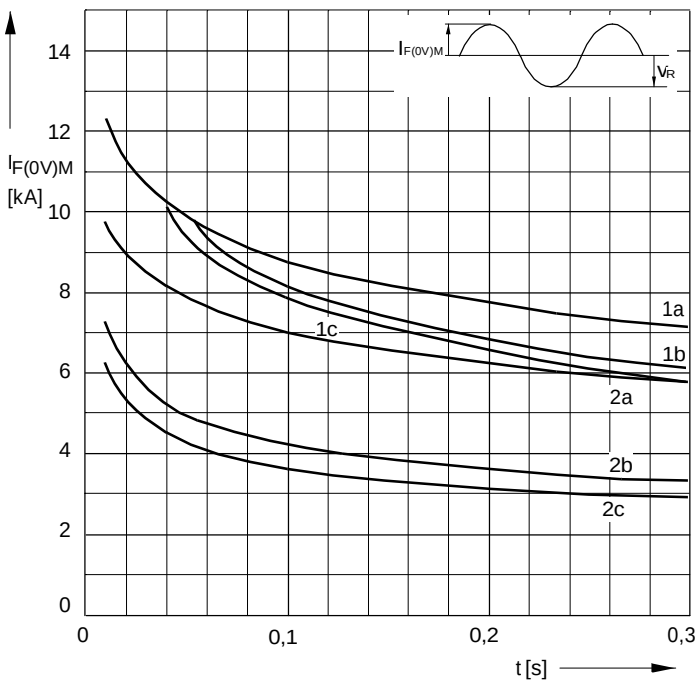
Bild / Fig. 3 Grenzstrom / Maximum overload forward current I_{F(0V)M} = f(t) 1 - I_{FAV(vor)} = 0\text{ A} ; t_{j} = t_c = 25\text{ °C} 2 - I_{FAV(vor)} = 400\text{ A} ; t_c = 130\text{ °C} ; t_{j} = 180\text{ °C} a - V_R \leq 50\text{ V} b - V_R = 0,5 V_{RRM} c - V_R = 0,8 V_{RRM}
