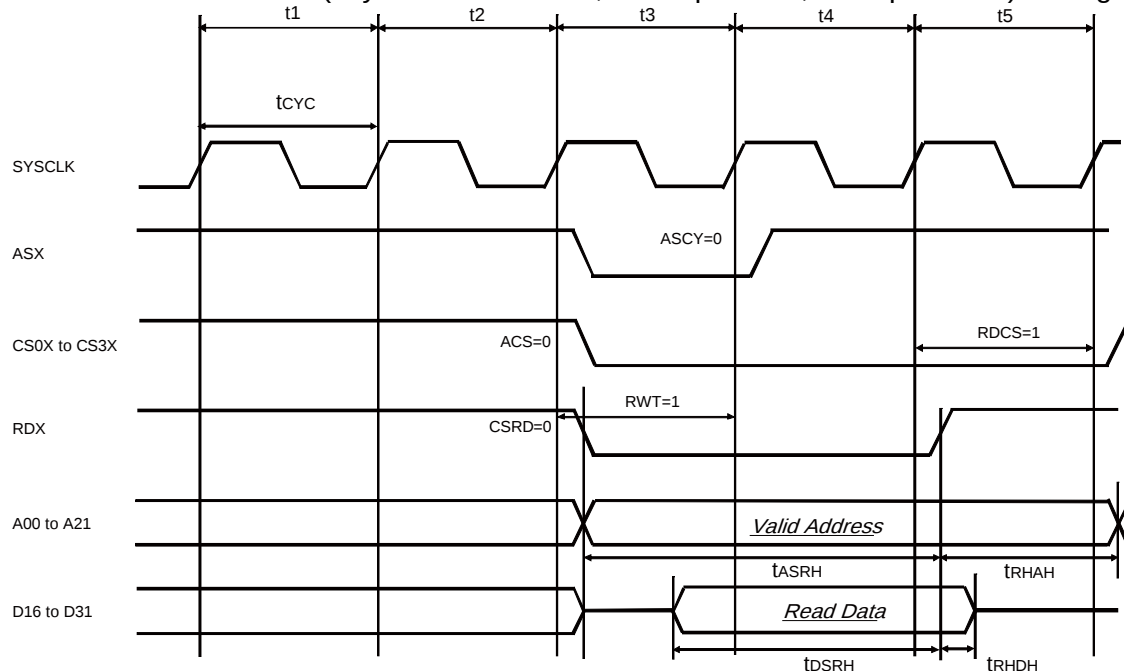
External bus I/F (asynchronous mode, read operation, and split mode) Timing
