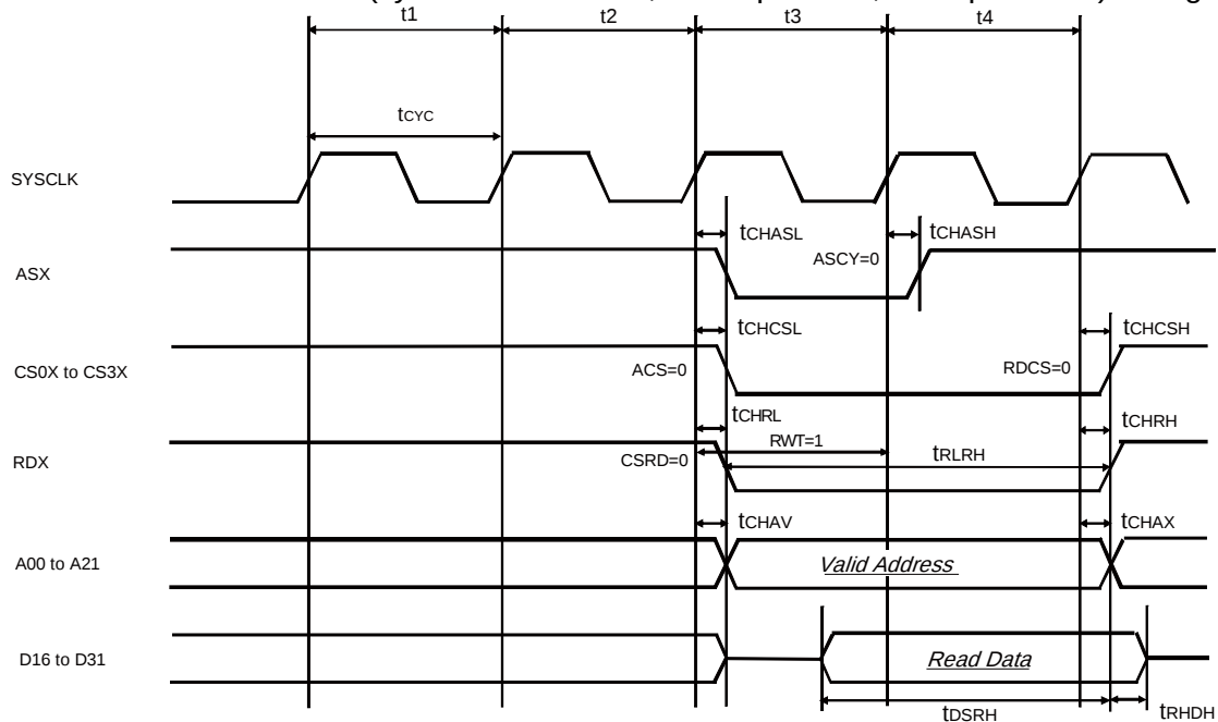
External bus I/F (synchronous mode, read operation, and split mode) timing
