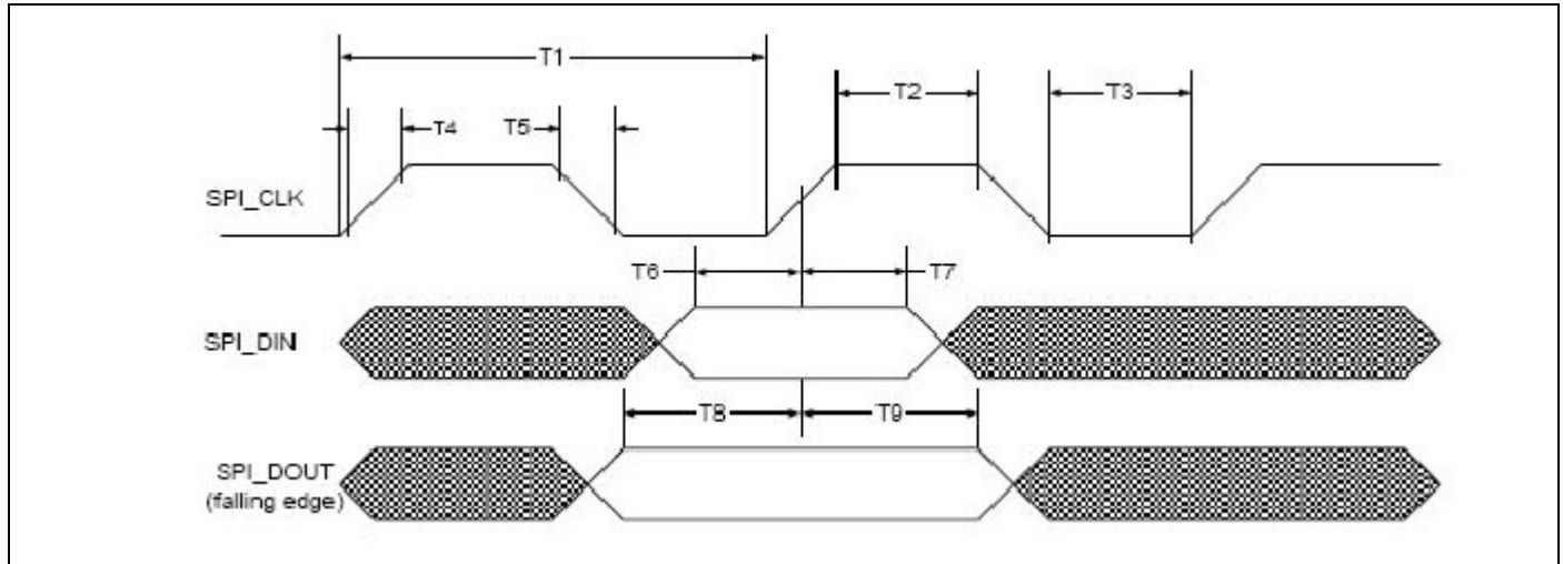
Figure 26. gSPI Timing
