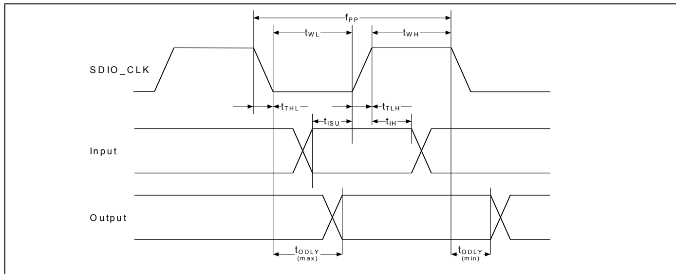
Figure 24. SDIO Bus Timing (Default Mode)
