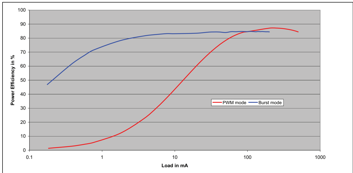
Figure 23. CBUCK Efficiency
