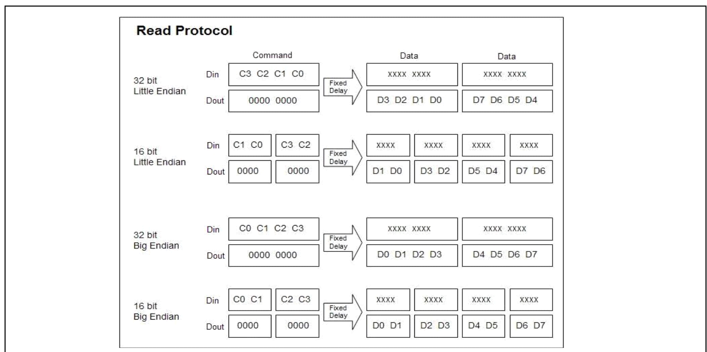
Figure 10. gSPI Read Protocol
