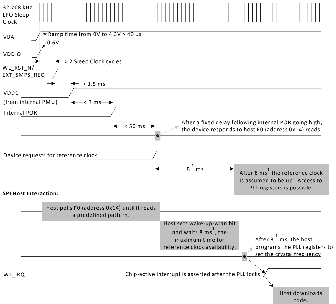
Figure 14. WLAN Boot-Up Sequence
