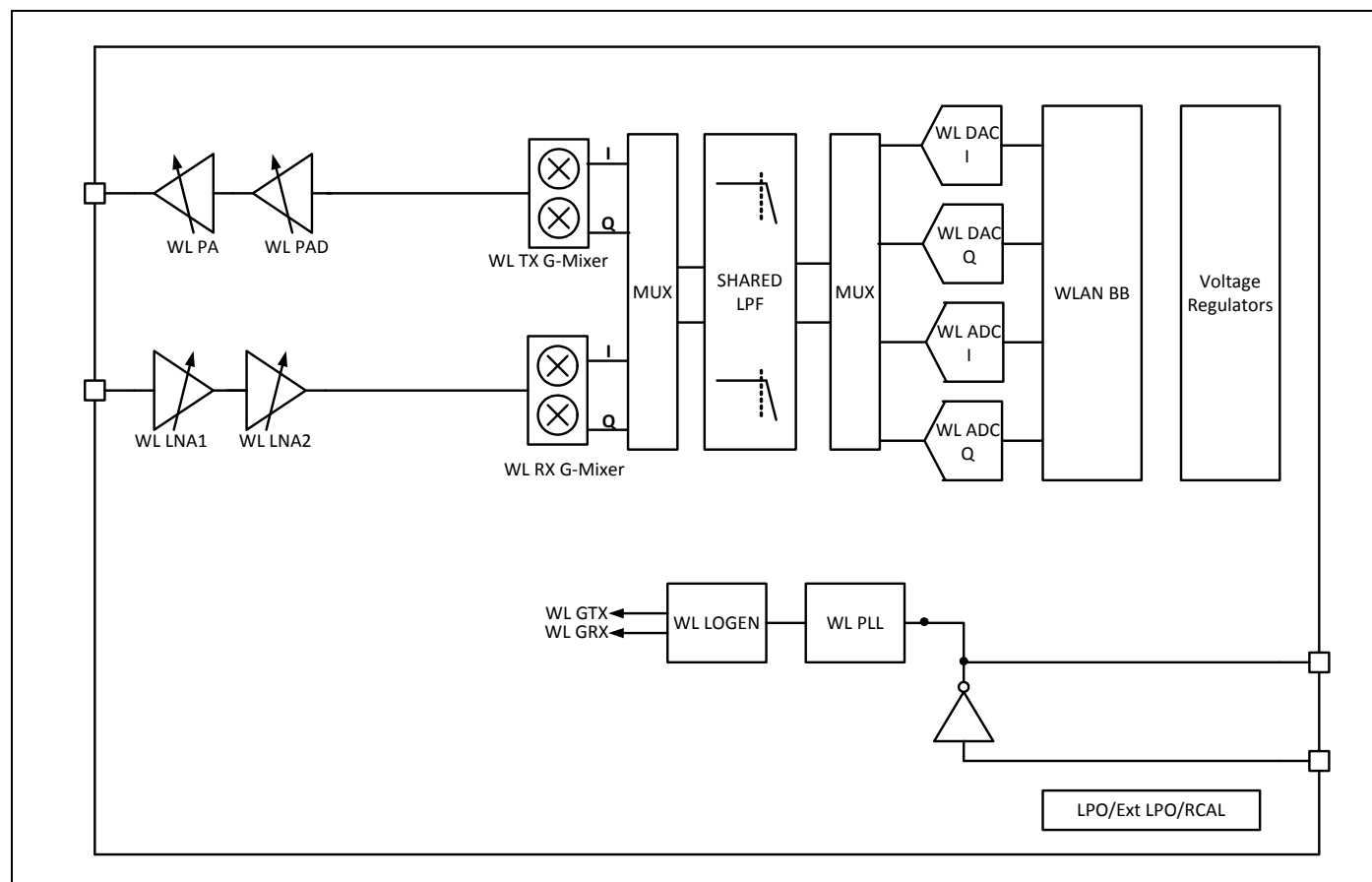
Figure 19. Radio Functional Block Diagram
