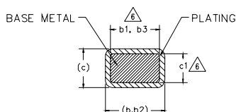
SECTION B-B & C-C
