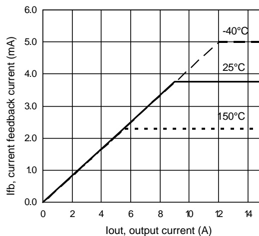
Figure 10 – I fb (mA) Vs I out (A)
