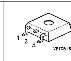
P-TO263-3-2
