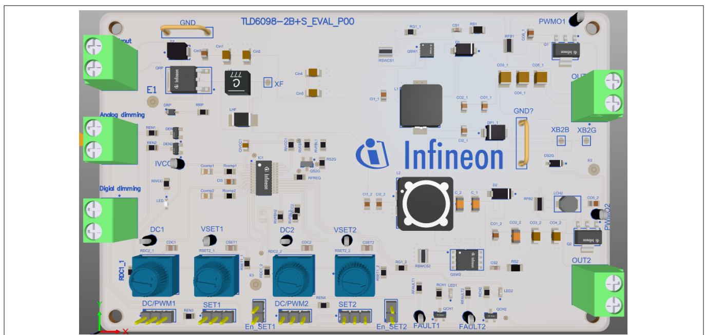
Figure 1 TLD6098 Boost and SEPIC Board
