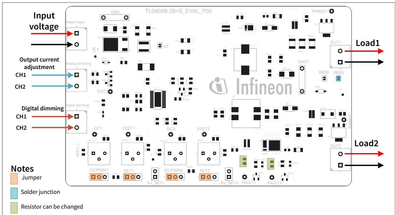
Figure 5 External dimming and output adjustment
