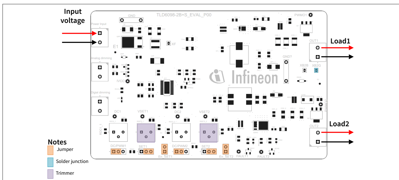
Figure 3 Current adjustment
