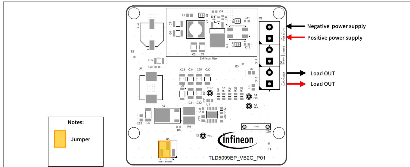
Figure 4 Auto-enable configuration
