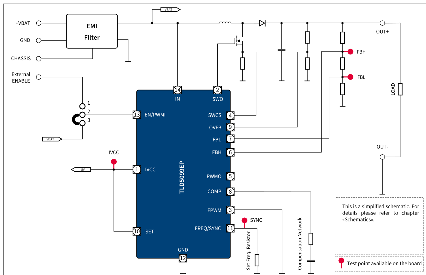
Figure 2 Simplified schematic
