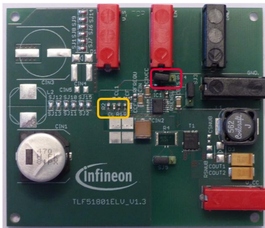
Figure 6 Adjustment of V_{OUT} and external BTS diode
