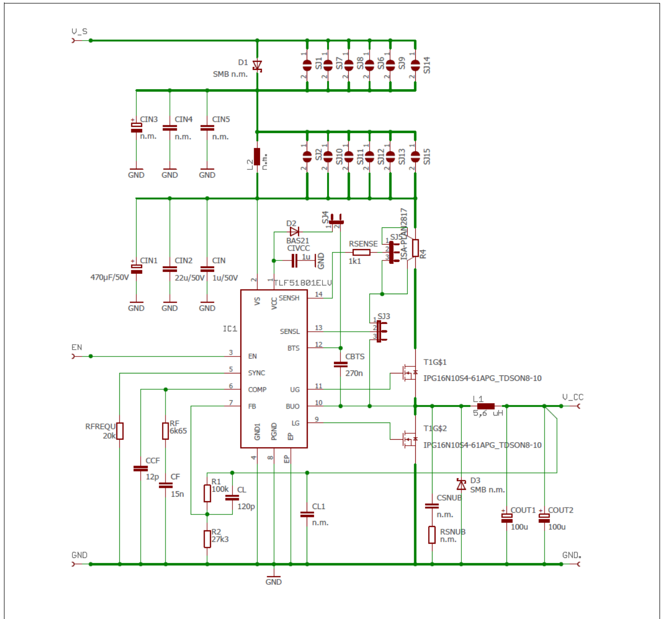
Figure 2 Demoboard schematic
