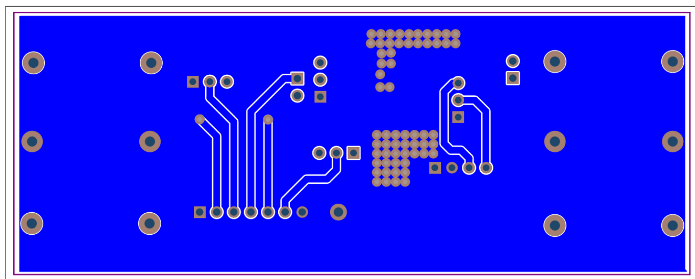
Figure 7 Bottom layer
