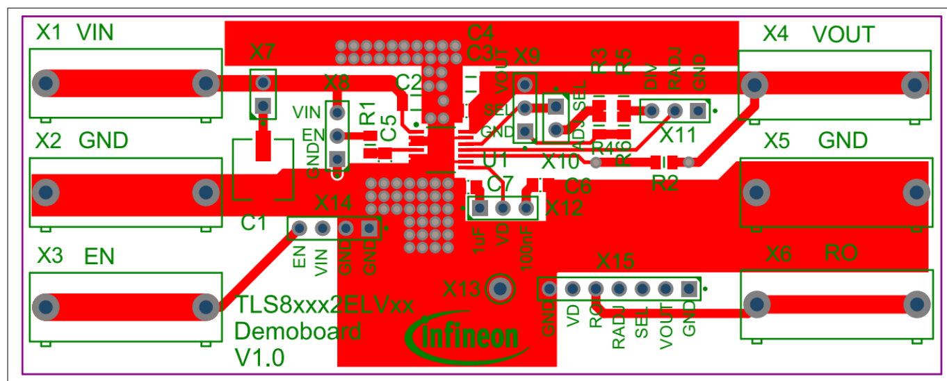
Figure 6 Top layer
