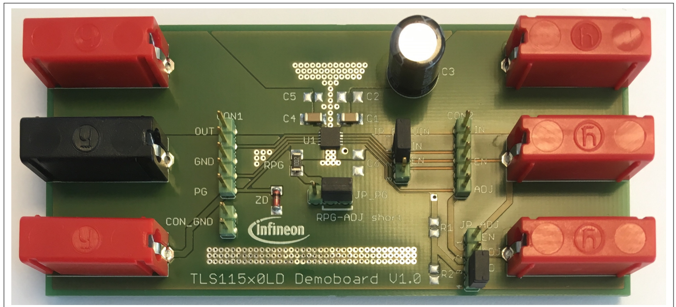
Figure 3 OPTIREG™ linear voltage regulator TLS115x0LD demoboard
