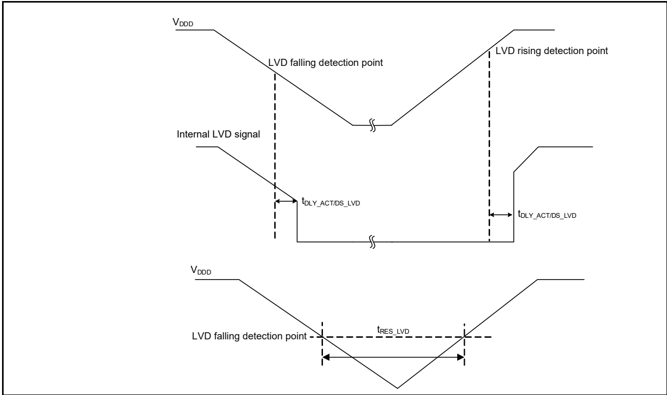
Figure 26-20 LVD specifications
