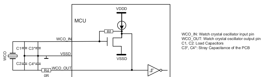
Figure 26-23 WCO connection scheme [68]
