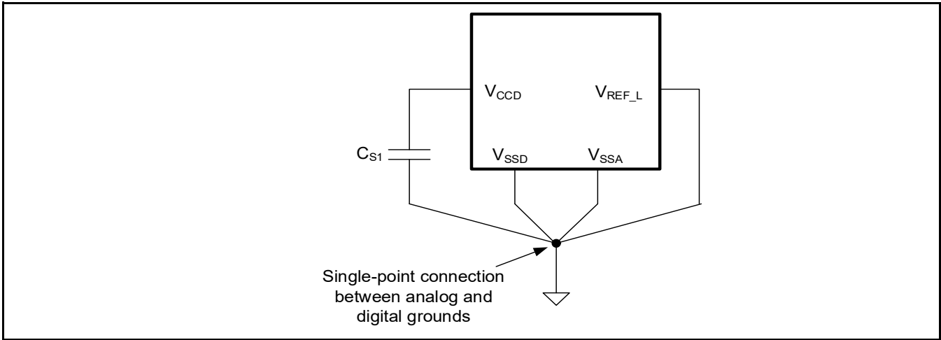
Figure 26-2 Smoothing capacitor
