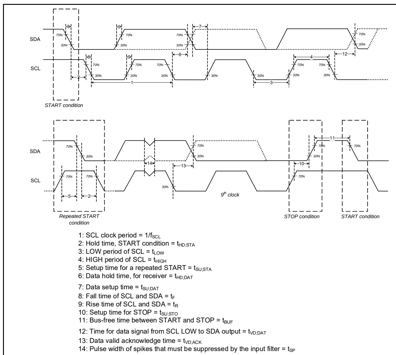
Figure 26-9 I²C timing diagrams
