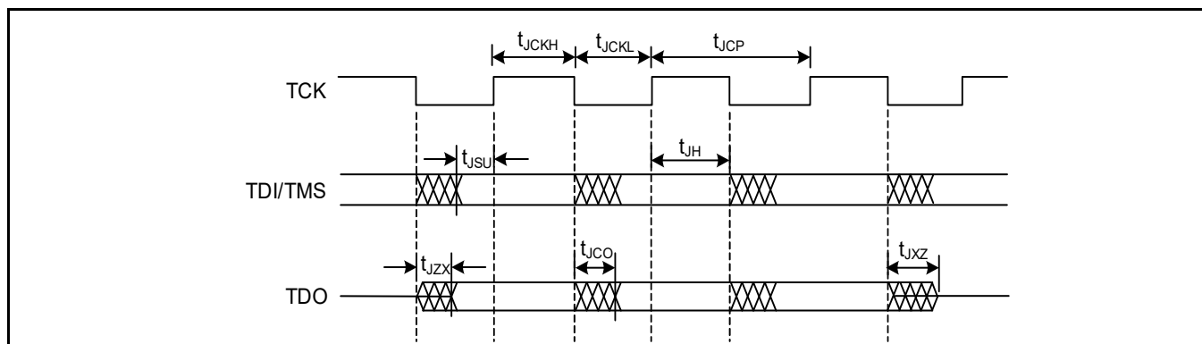
Figure 26-21 JTAG specifications
