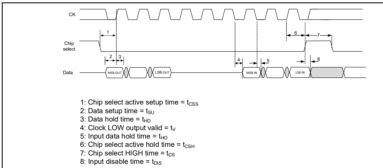
Figure 26-35 SDR write and read timing diagram
