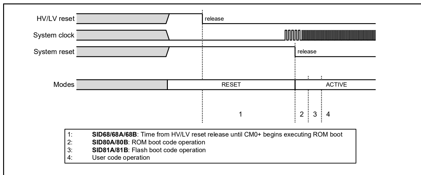
Figure 26-3 Reset sequence
