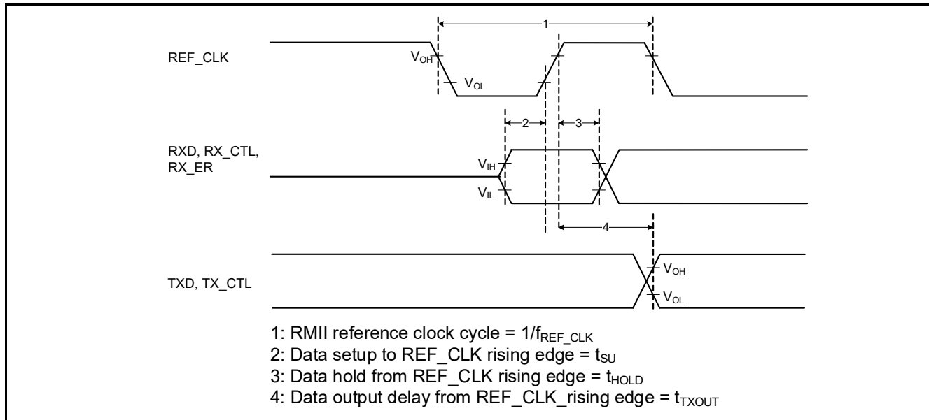
Figure 26-28 RMII timing diagram
