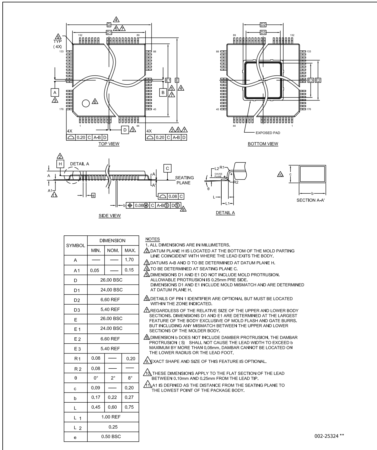
Figure 28-1 Package outline – 176-TQFP
