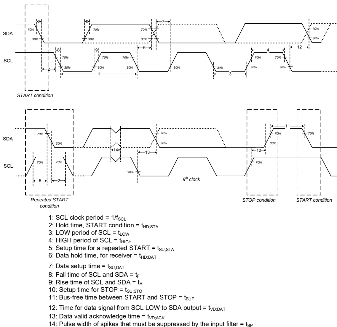
Figure 26-9 I 2 C timing diagrams
