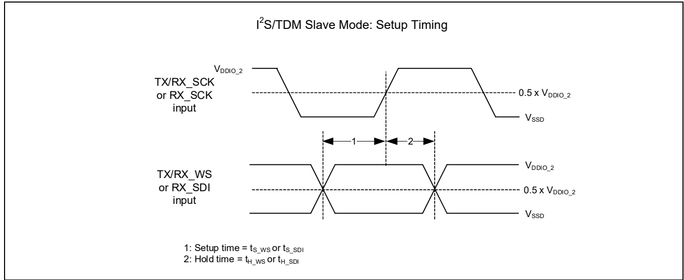
Figure 26-39 Slave setup
