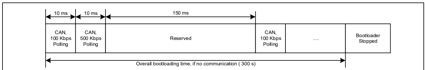
Figure 29-1 Bootloading sequence
