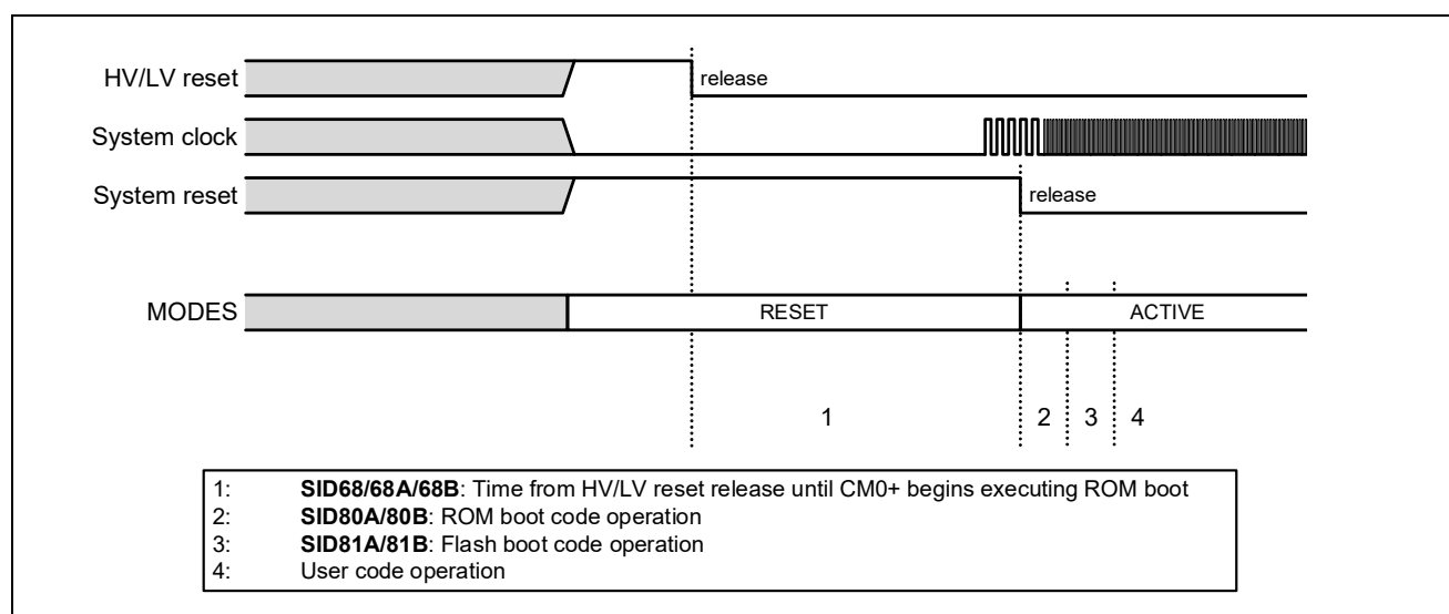
Figure 26-3 Reset sequence
