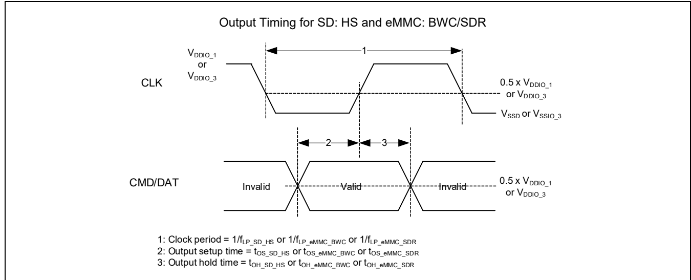
Figure 26-32 SD high-speed and eMMC BWC/SDR output timing
