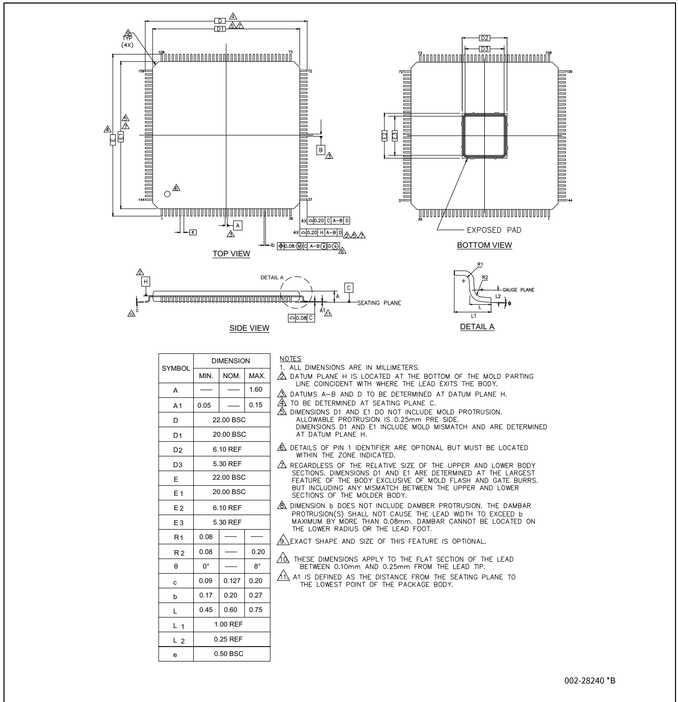
Figure 28-2 Package outline – 144-TQFP
