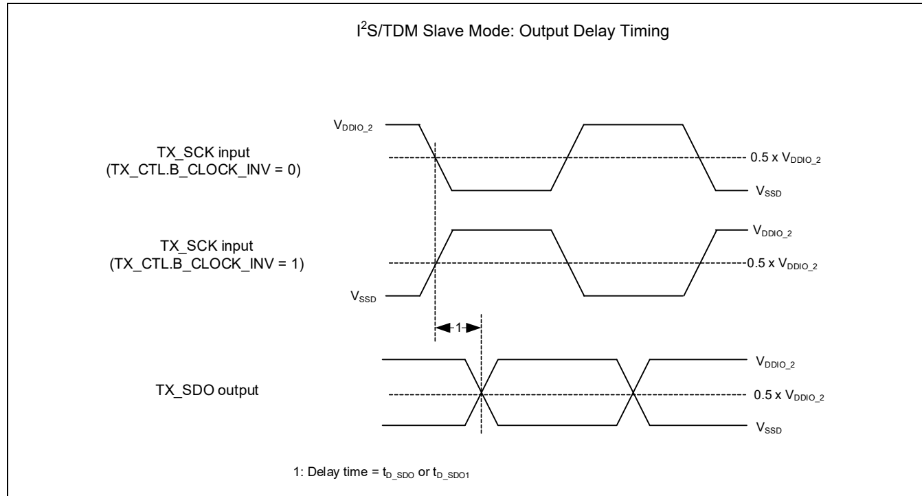
Figure 26-38 Slave output delay
