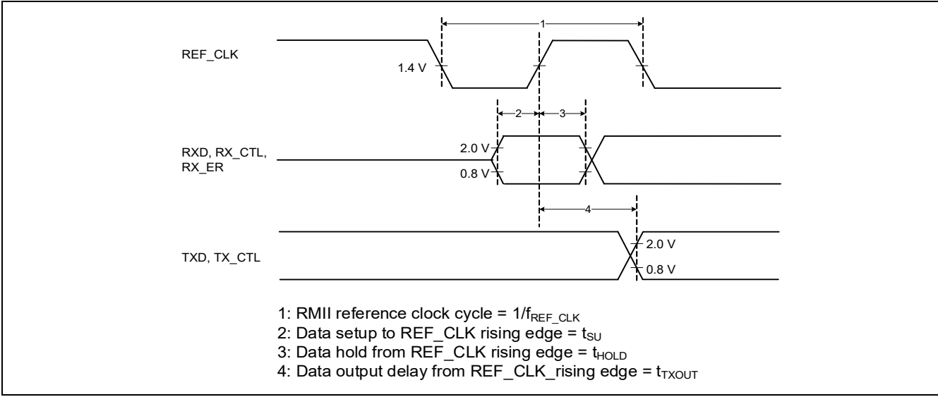
Figure 26-28 RMII timing diagram
