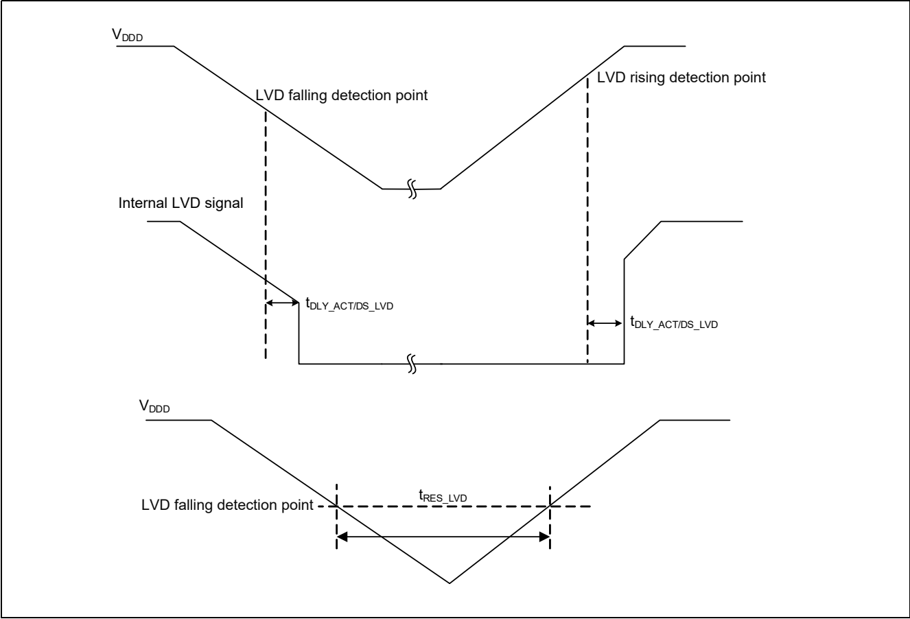
Figure 26-20 LVD specifications
