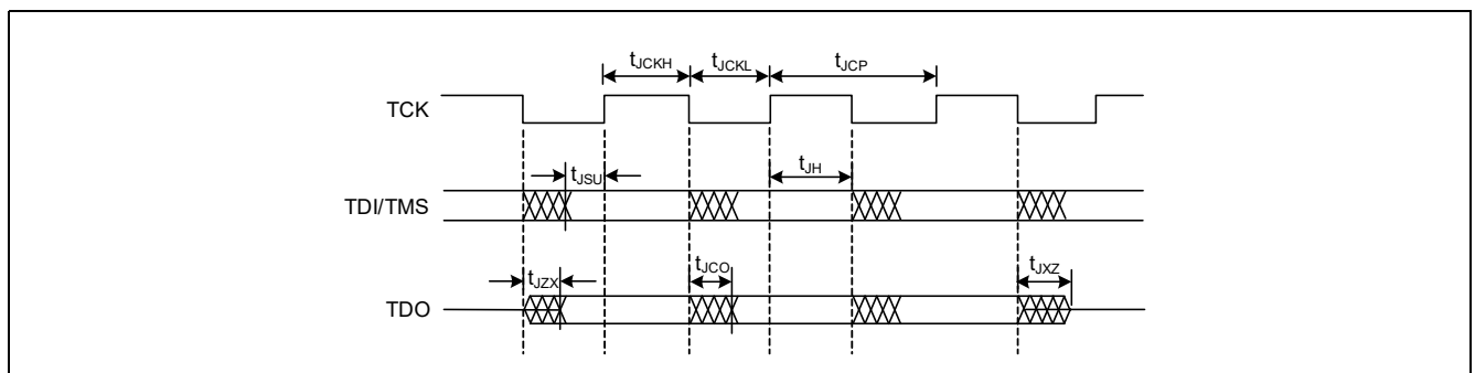
Figure 26-21 JTAG specifications
