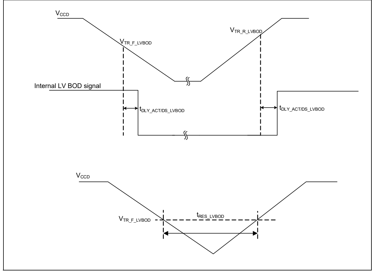
Figure 26-17 Low-voltage BOD specifications
