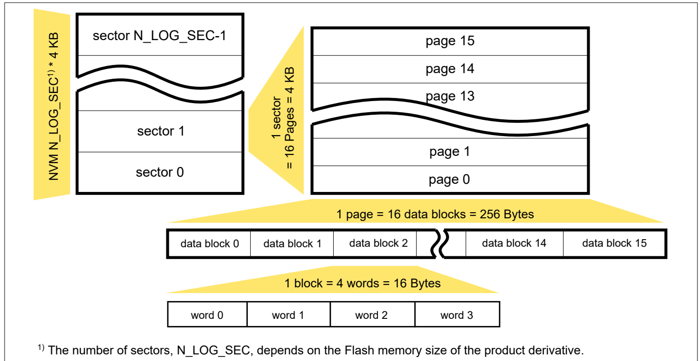
Figure 19 Logical Structure of the Flash
