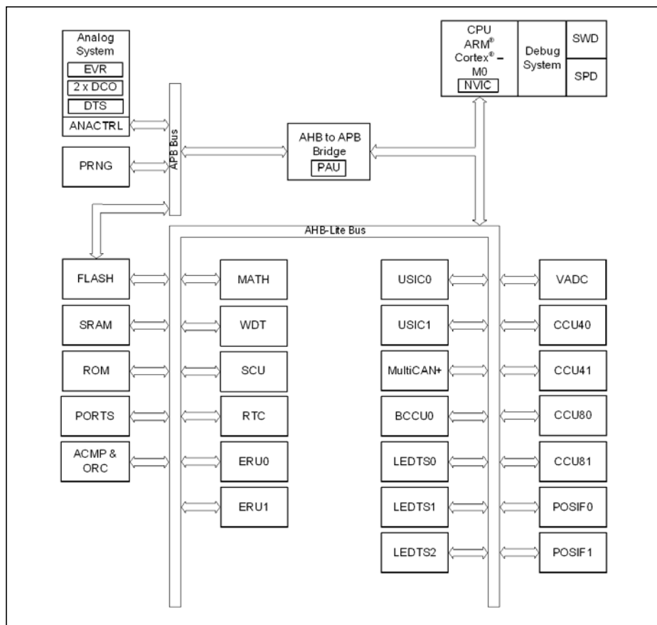
Figure 1 Block Diagram
