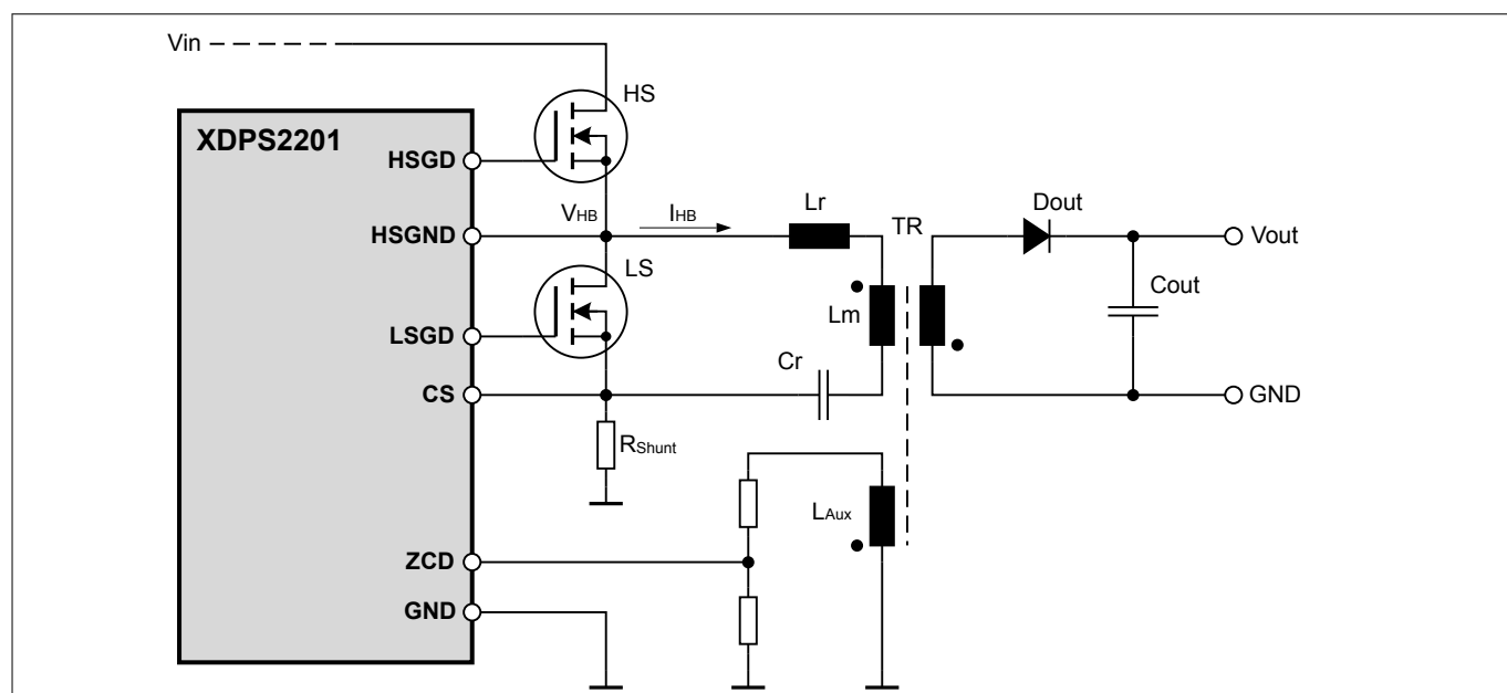
Figure 4 Hybrid-flyback power stage
