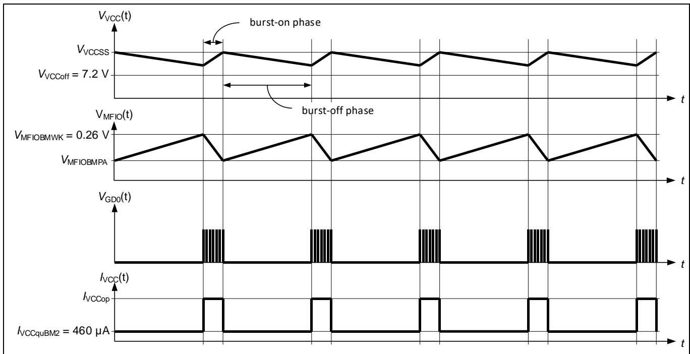
Figure 7 Burst operation
