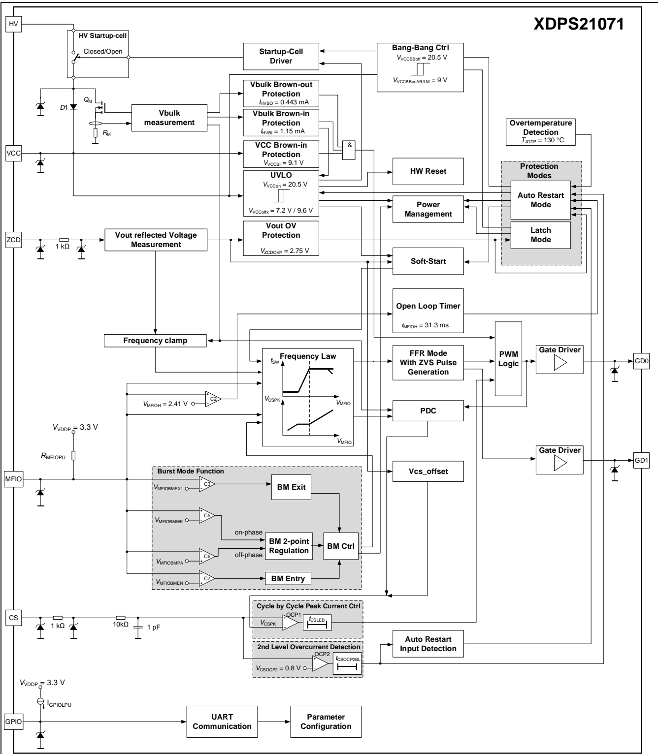
Figure 3 Representative Block Diagram of XDPS21071
