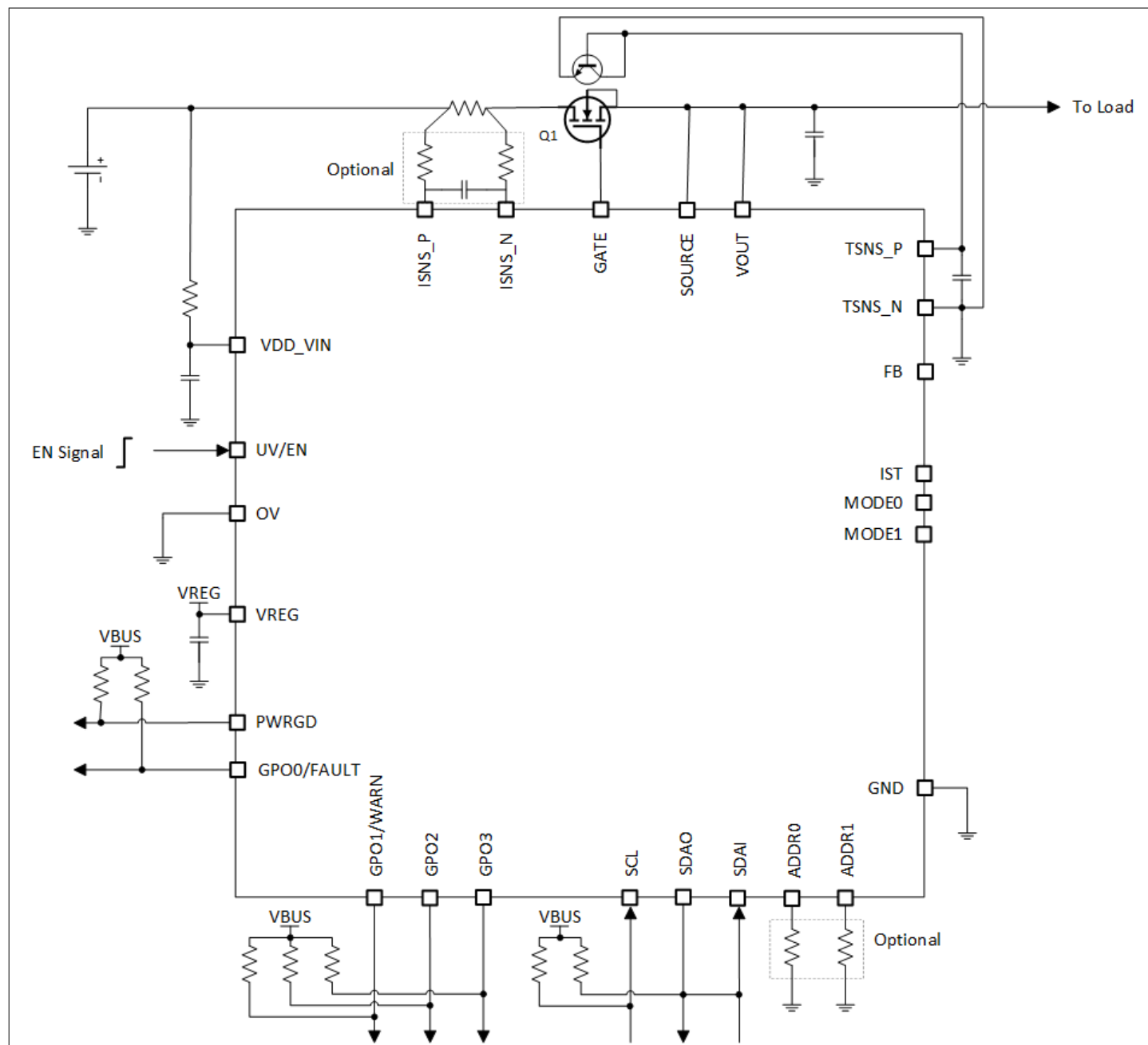
Figure 31 Fully digital mode DCM (MODE:MODE=0x1) application schematic
