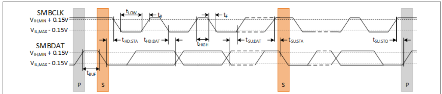
Figure 12 PMBus timing diagram
