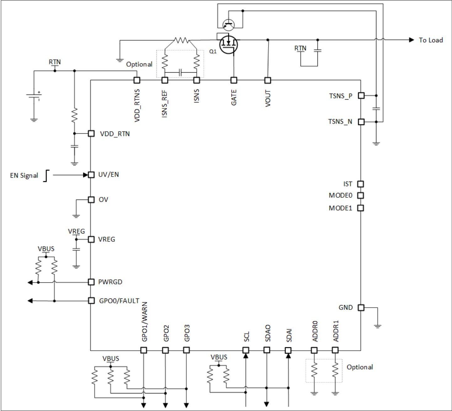
Figure 32 Fully digital mode DCM (MODE:MODE=0x1) application schematic
