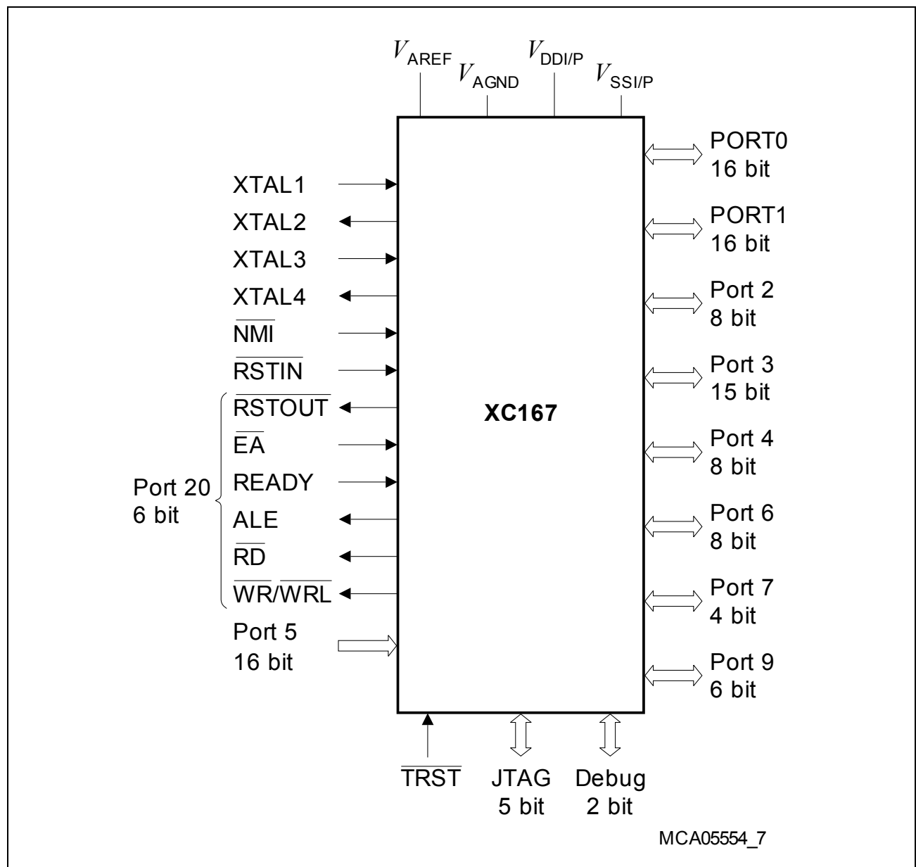
Figure 1 Logic Symbol
