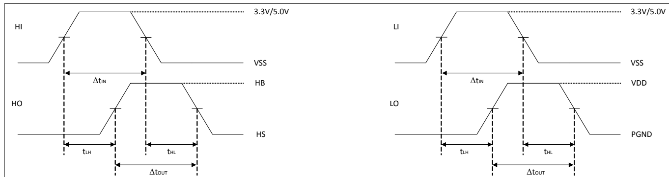
Figure 4 Propagation delay
