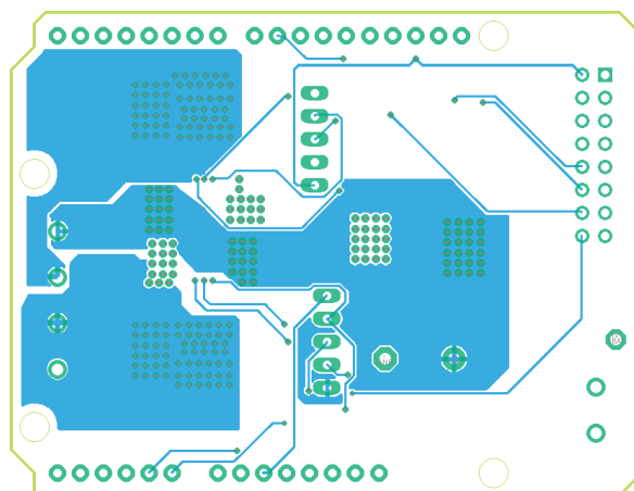
Figure 14 Bottom layer, bottom view rev. 1.2
