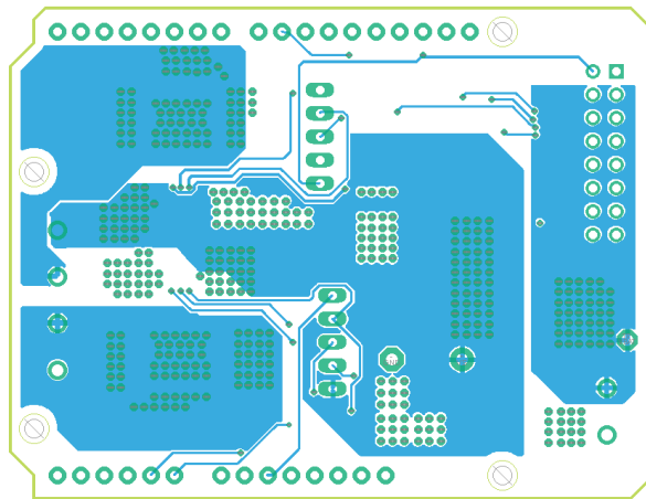
Figure 19 Bottom layer, bottom view rev. 2.0
