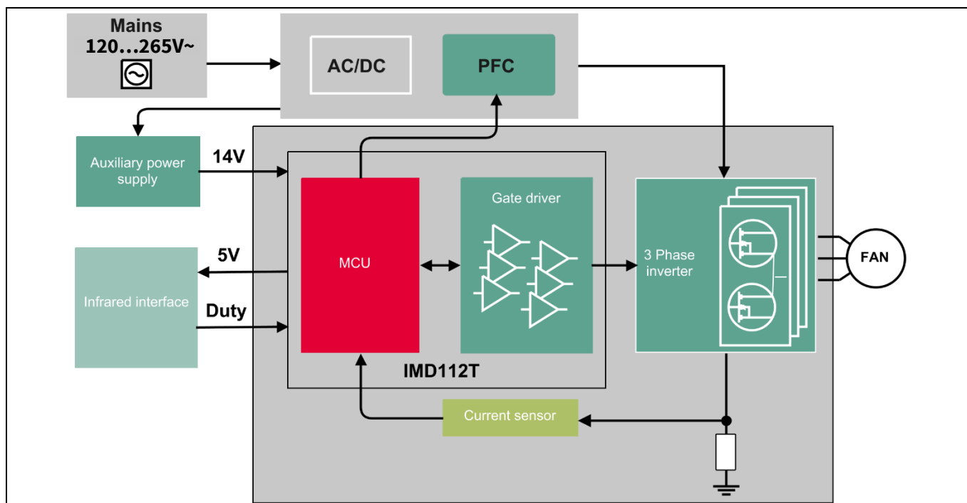
Figure 1 Block diagram of the REF-SHA35WRC2SYS
