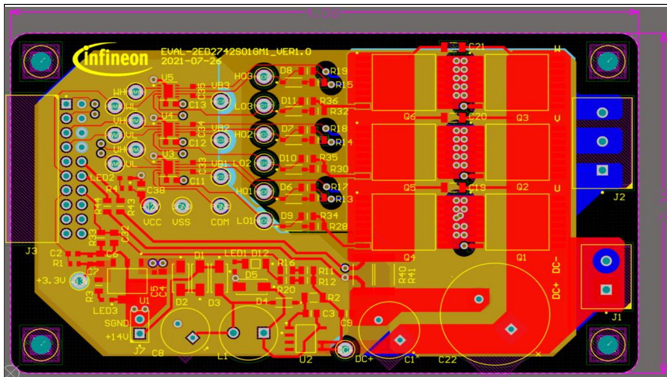
Figure 19 Power inverter board layout (All 4 layers together)
