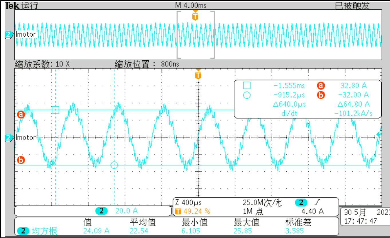
Figure 26 Current at light load
