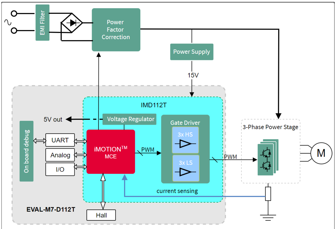
Figure 2 Block diagram of EVAL-M7-D112T
