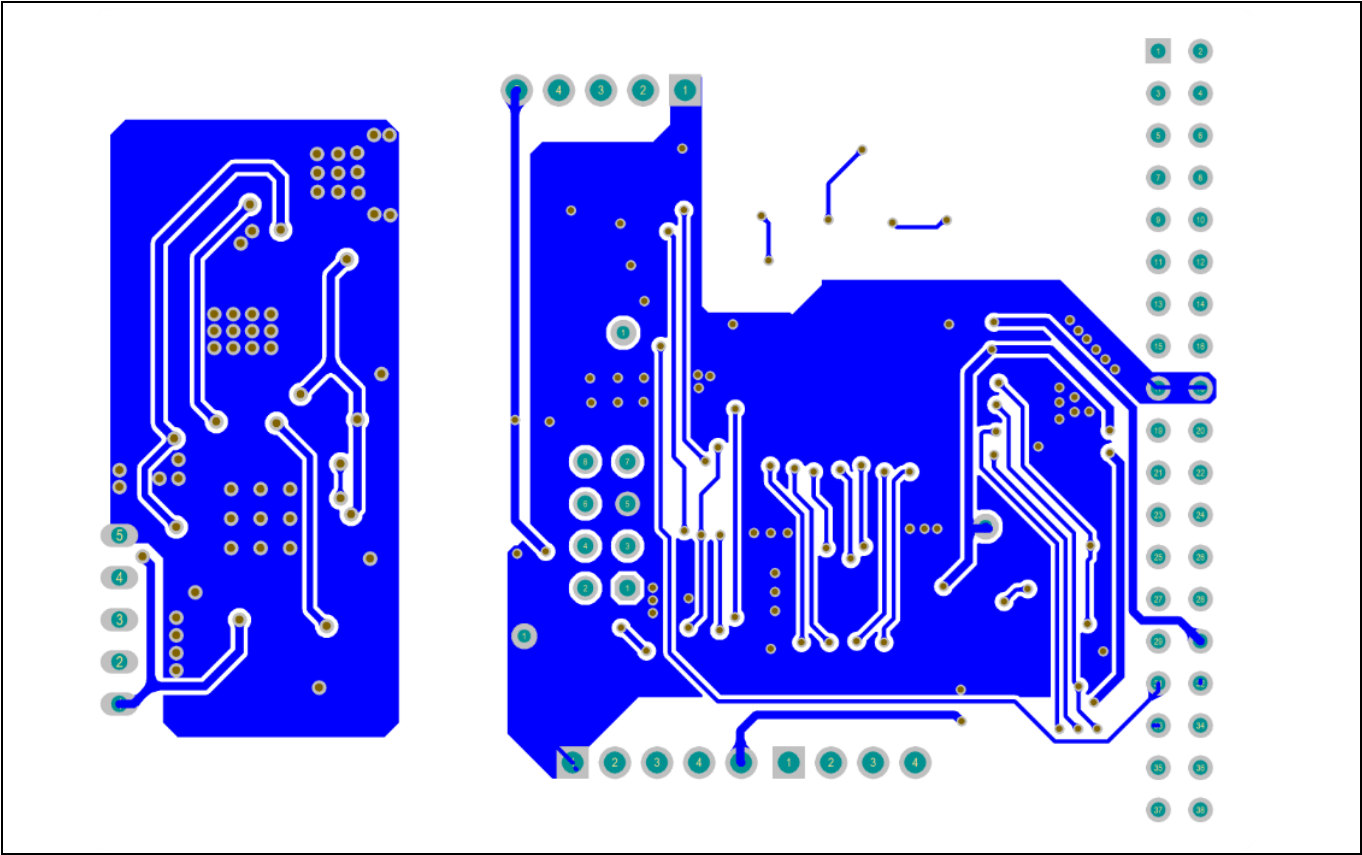
Figure 11 Bottom layer
