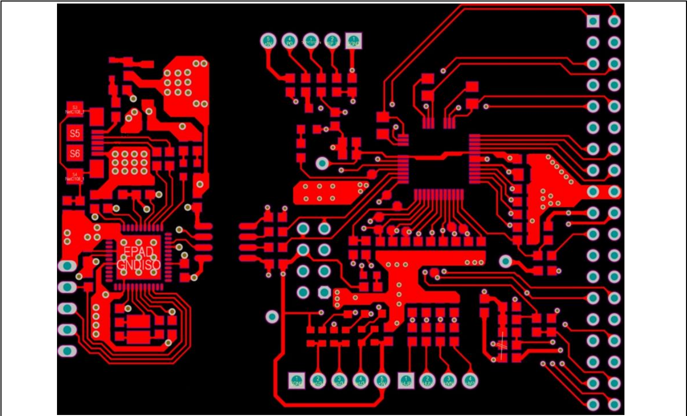
Figure 10 Top layer
