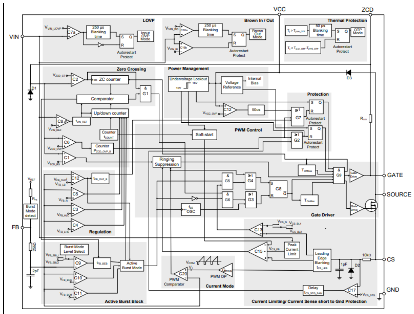
Figure 10 Circuit diagram
