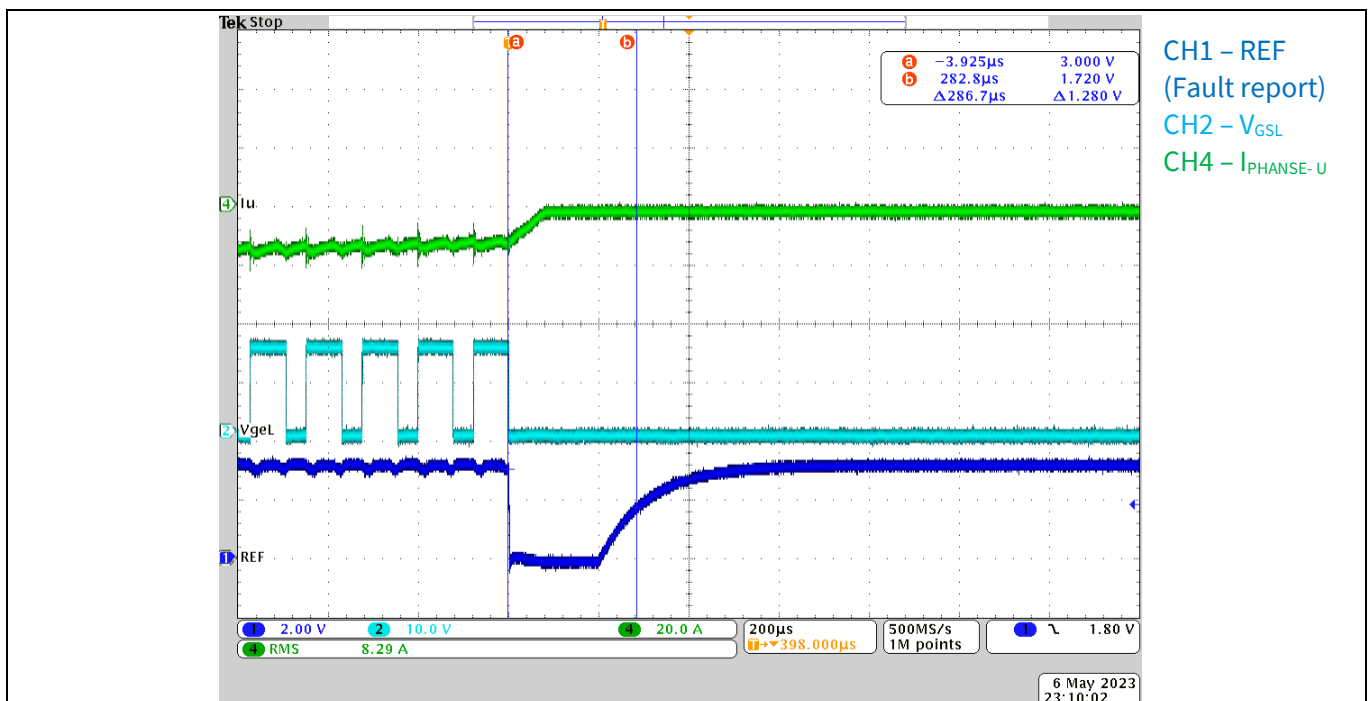
Figure 25 Overcurrent protection
