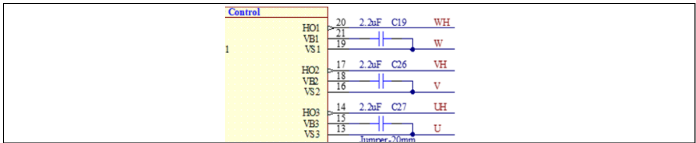
Figure 21 Bootstrap capacitors
