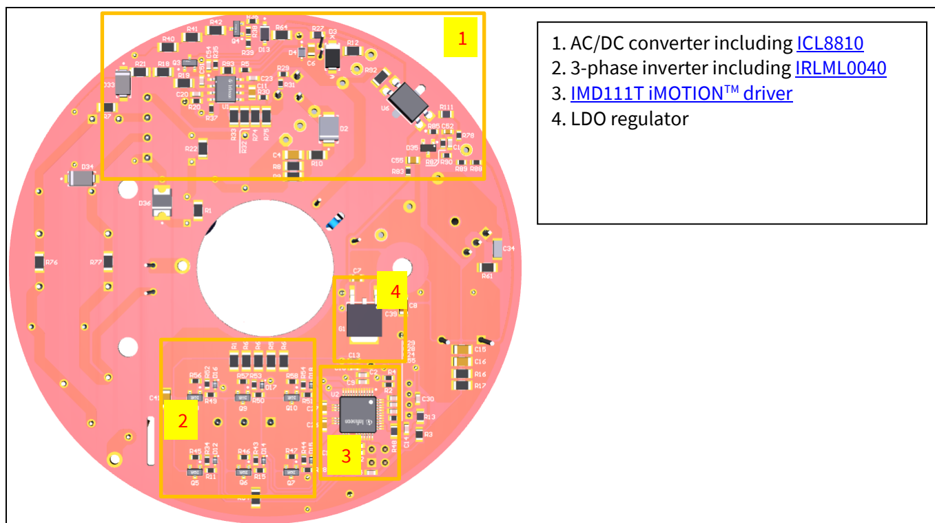
Figure 3 REF-SHA35IMD111TSYS - bottom side
