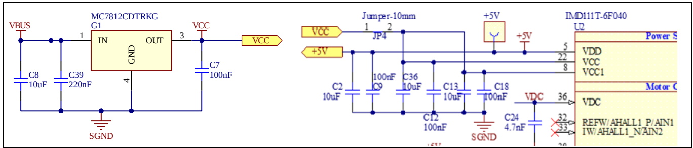
Figure 20 Power supply of IMD11T-6F064
