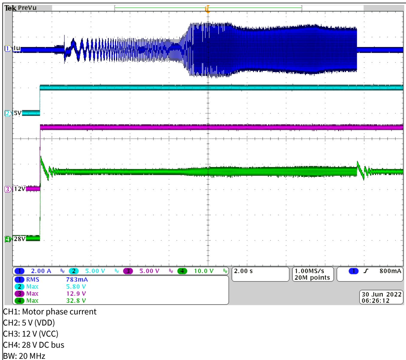
Figure 30 28 V, 12 V, and 5 V regulations at 230 V rms power ON/OFF at maximum speed
