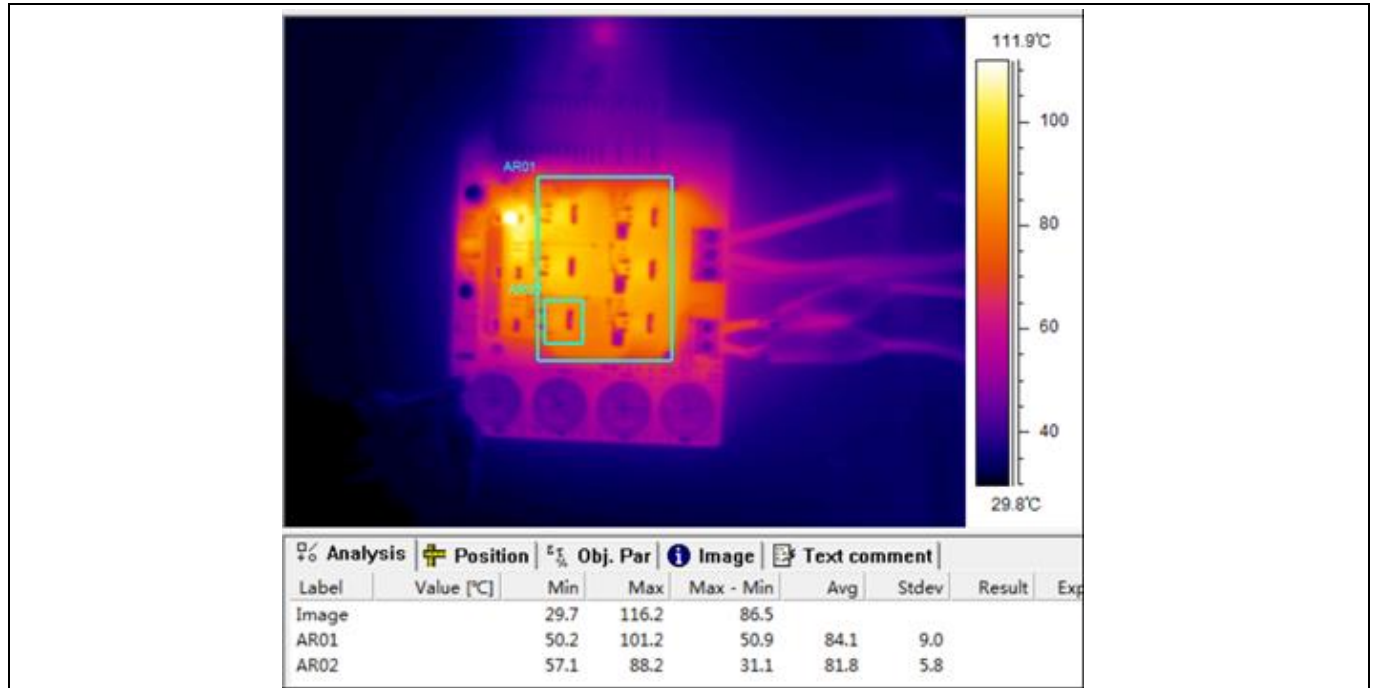
Figure 20 Thermal test
