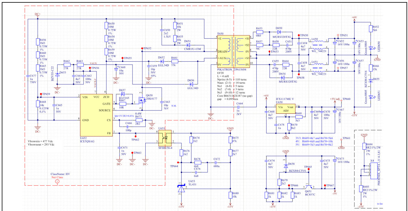
Figure 14 Auxiliary supply
