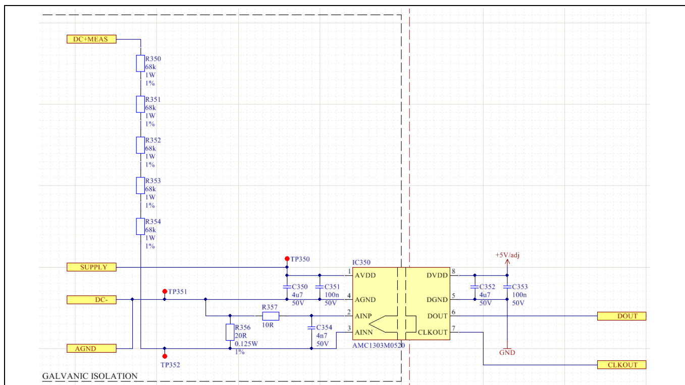
Figure 23 DC-bus voltage measurement
