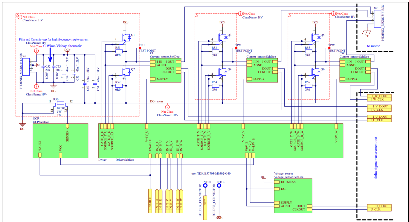
Figure 16 Power stage
