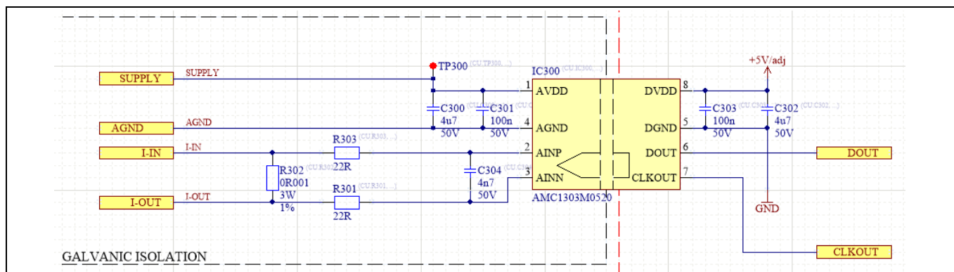
Figure 22 Phase current measurement
