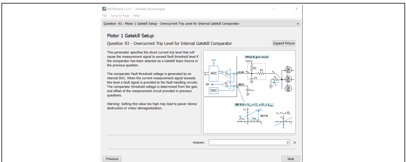
Figure 14 Over current trip level setting in MCEWzard
