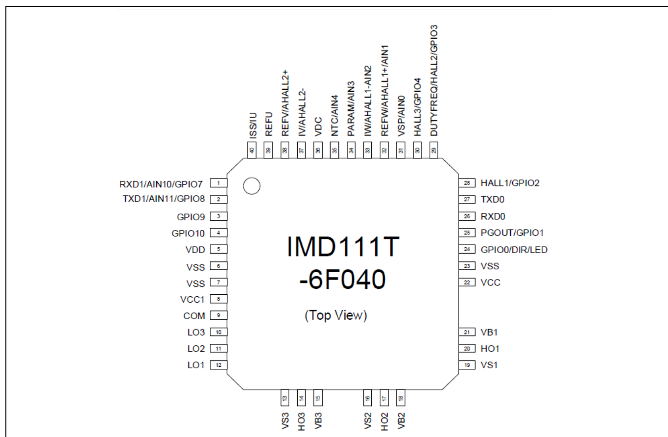
Figure 9 IMD111T pinout
