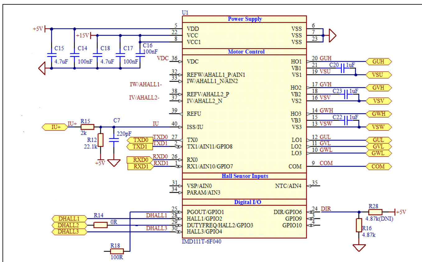
Figure 11 IMD111T schematics
