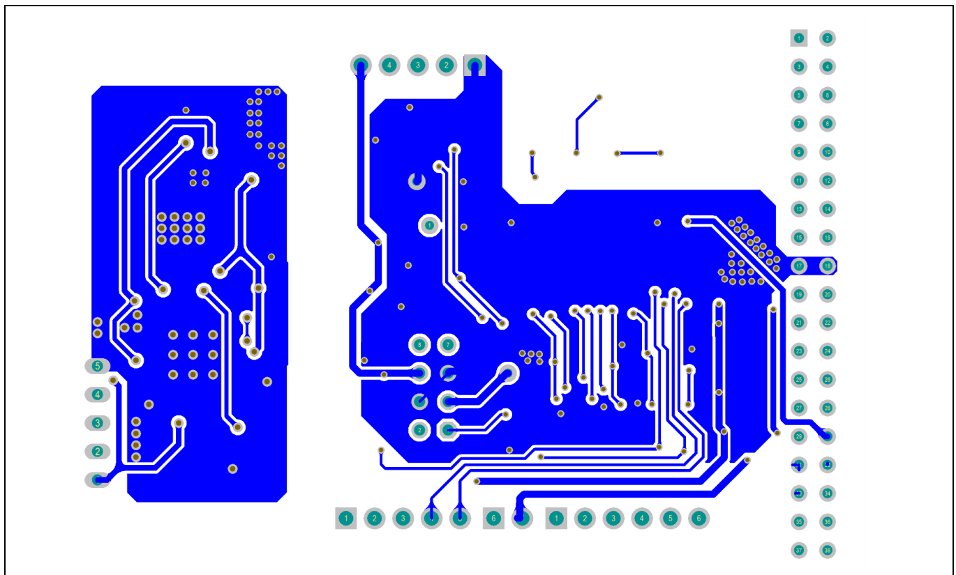
Figure 13 Bottom layer
