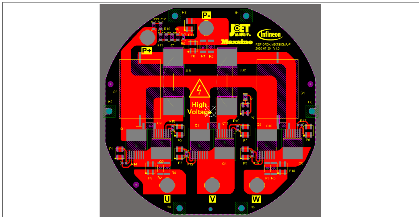
Figure 9 The layout of the power board (REF-DR3KIMBGSICMA-P)
