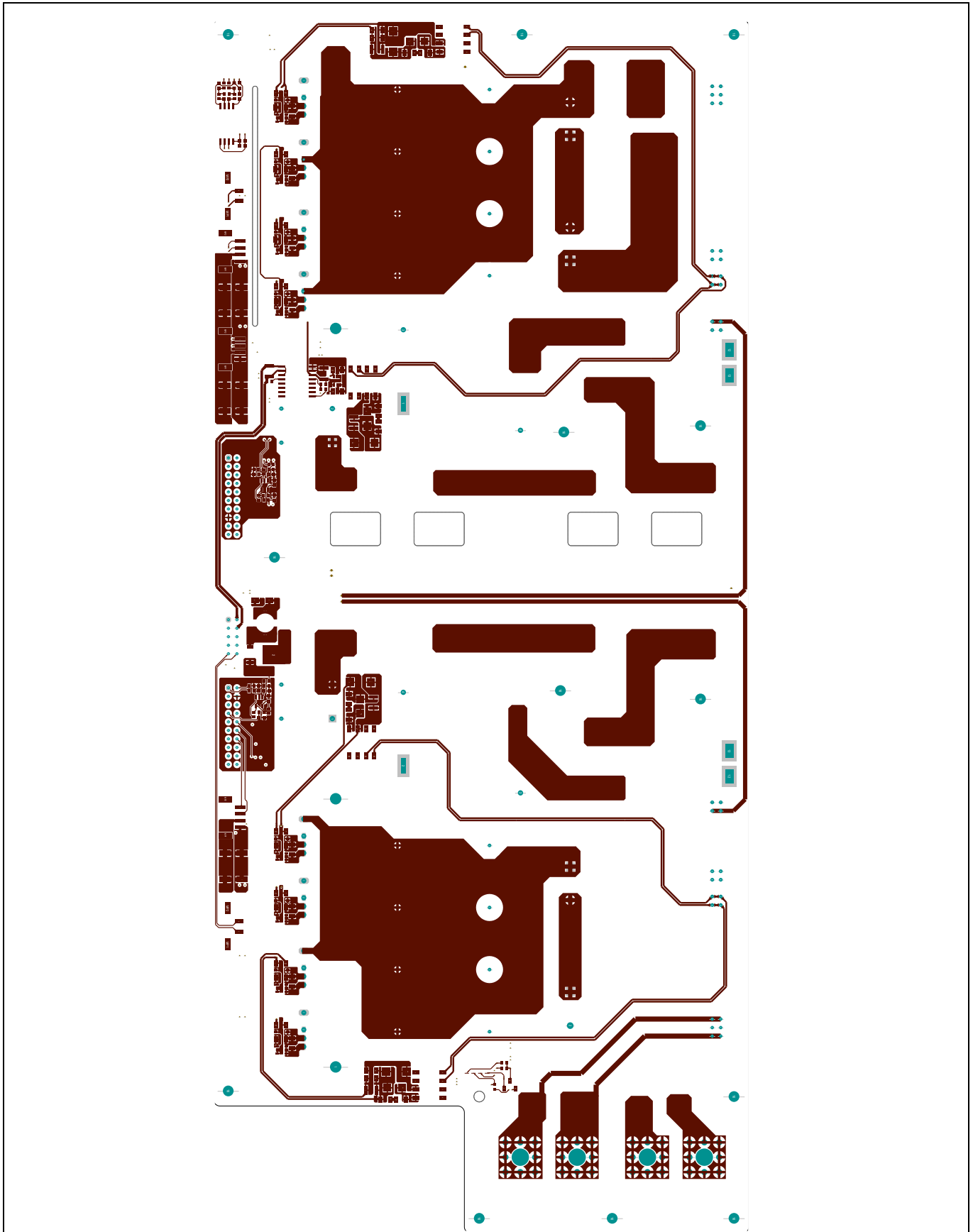
Figure 30 Top Layer
