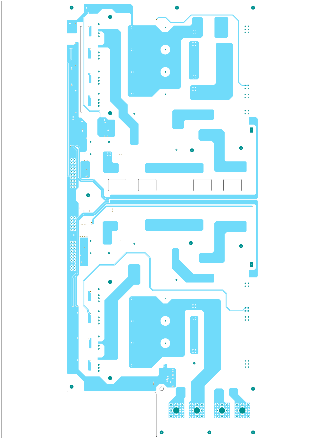
Figure 32 Layer 3
