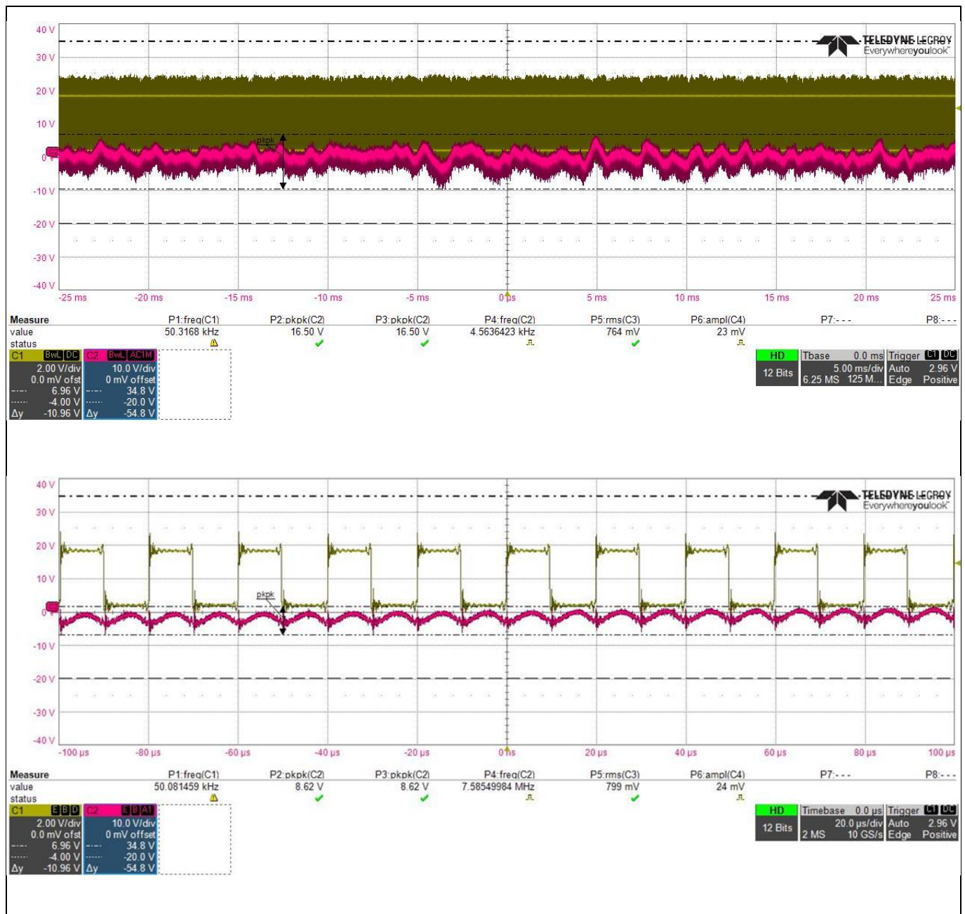
Figure 13 Output voltage ripple
