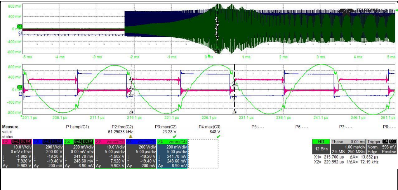
Figure 10 Test result of added sudden load
