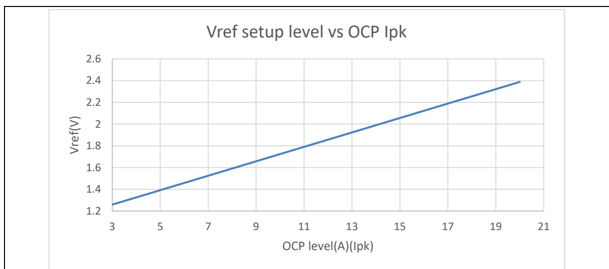
Figure 30 Vref vs overcurrent ( I_{OCP} )
