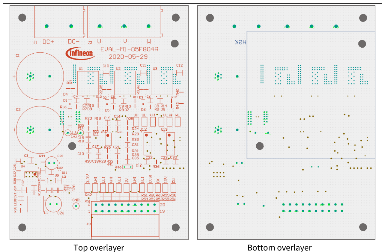
Figure 37 PCB overlayer
