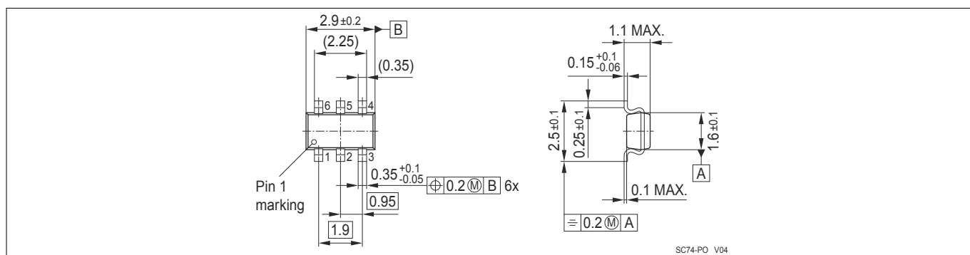
Figure 15 SC74-6-2 package outline
