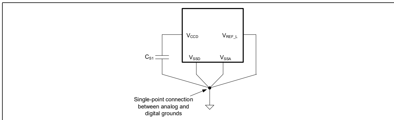
Figure 27-2 Smoothing capacitor
