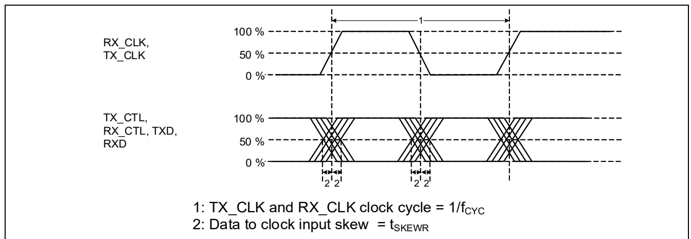
Figure 27-31 RGMII Rx timing diagram
