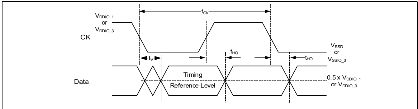
Figure 27-46 DDR read timing reference level
