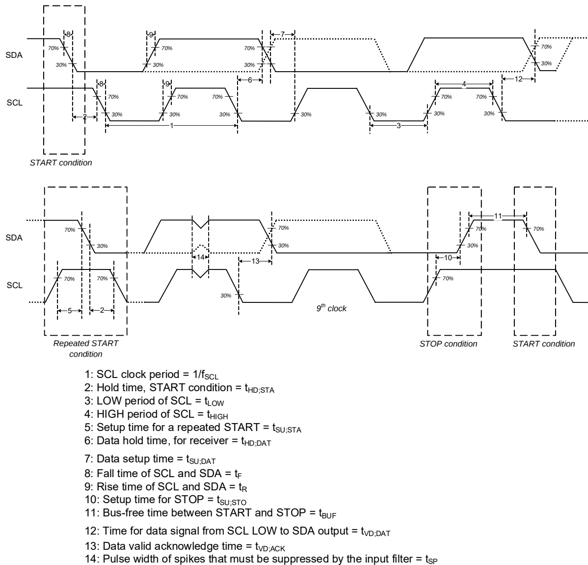
Figure 27-9 I 2 C timing diagrams
