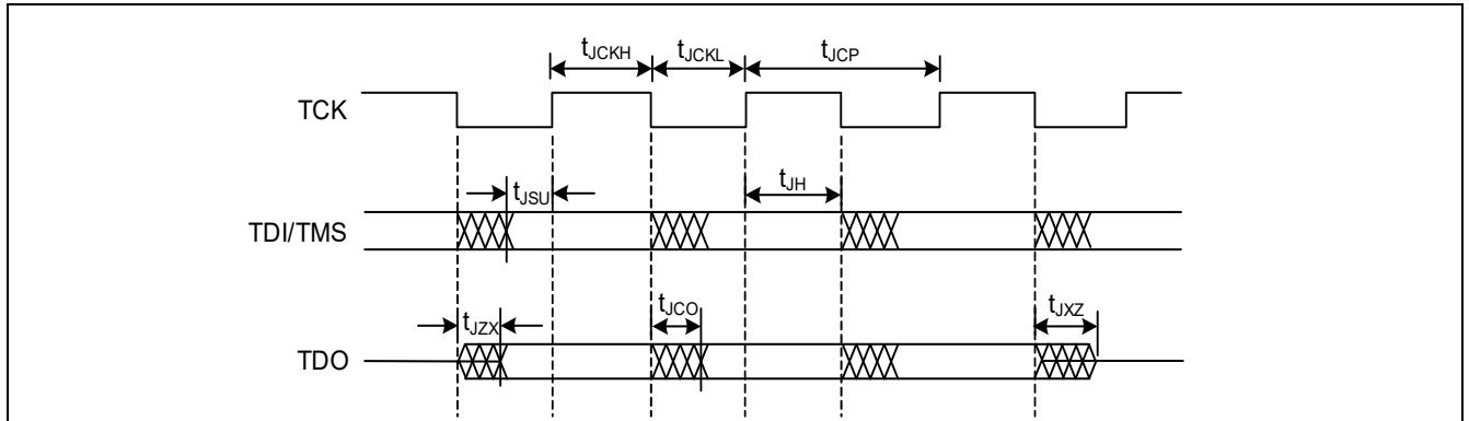
Figure 27-21 JTAG specifications
