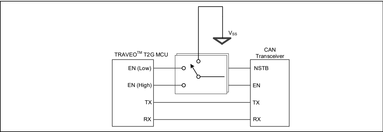
Figure 29-2 MCU to CAN transceiver connections
