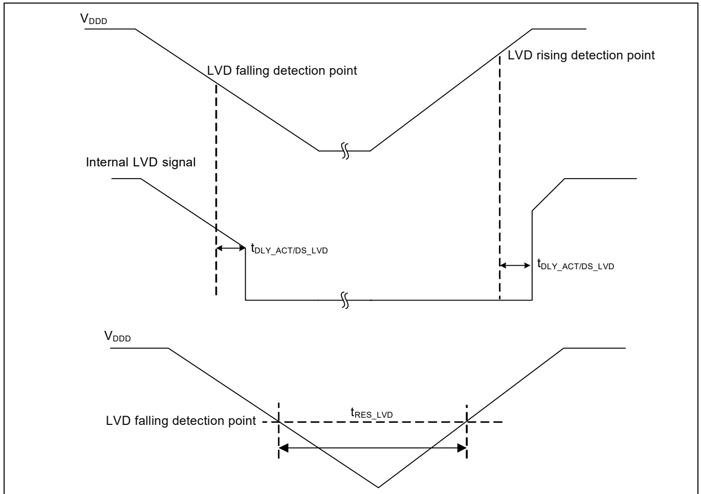
Figure 27-20 LVD specifications
