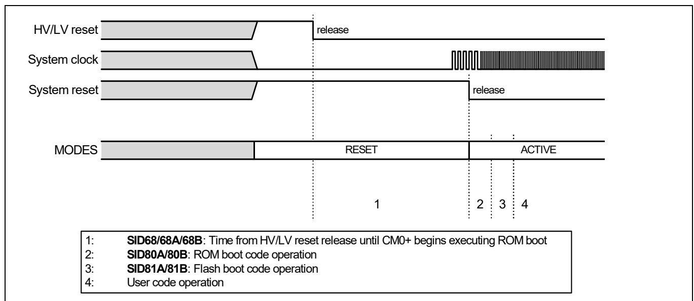
Figure 27-3 Reset sequence
