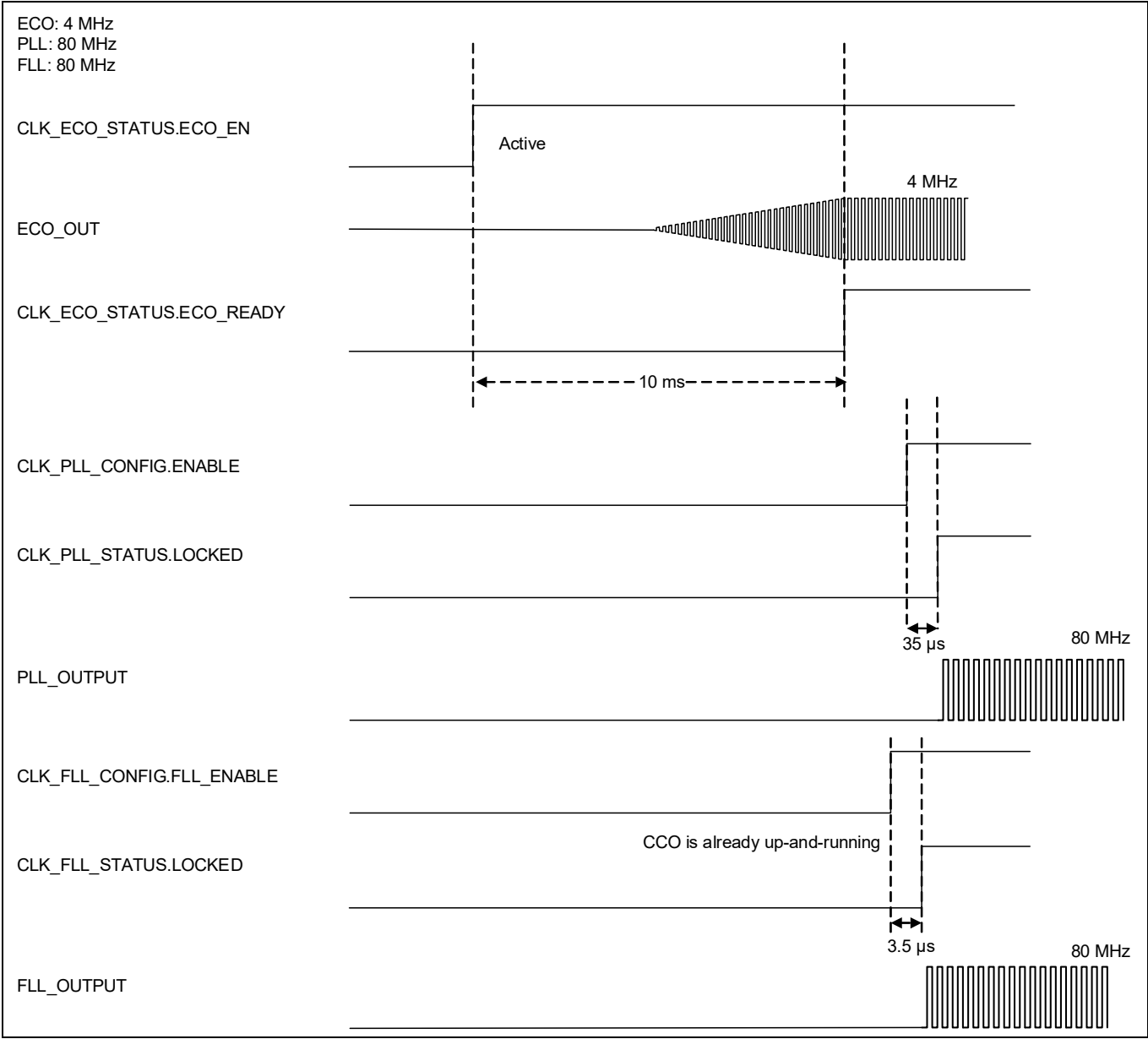
Figure 27-24 ECO to PLL or FLL diagram
