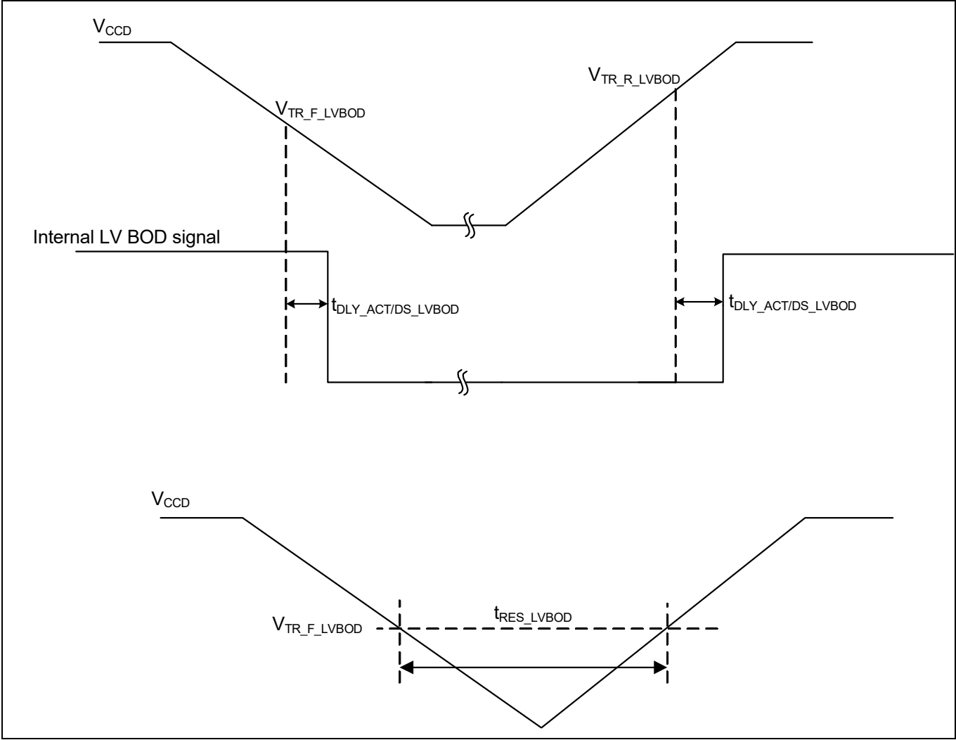
Figure 27-17 Low-voltage BOD specifications
