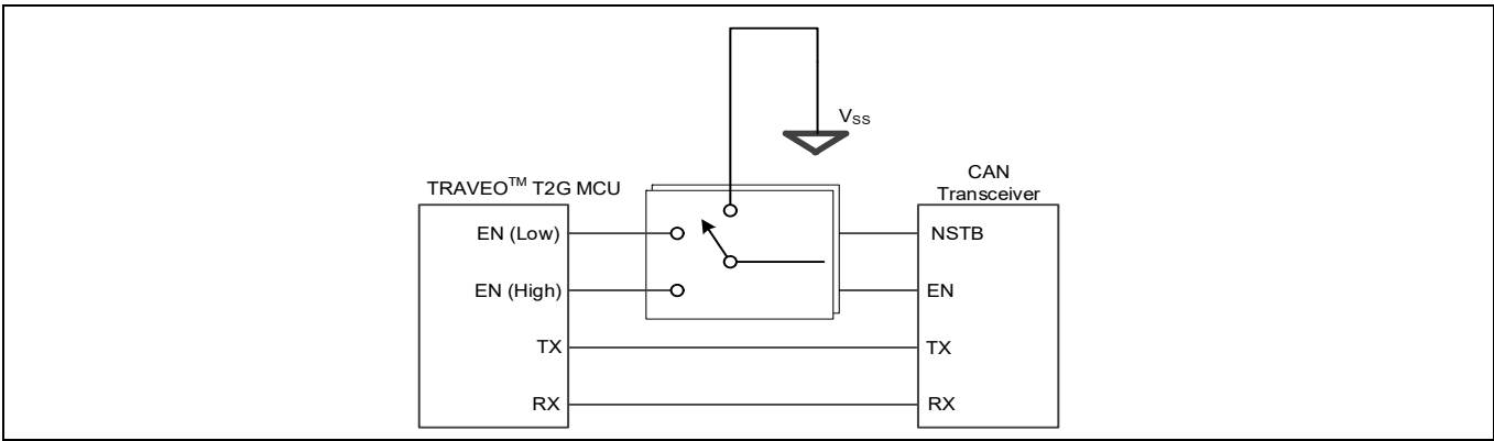
Figure 30-2 MCU to CAN transceiver connections
