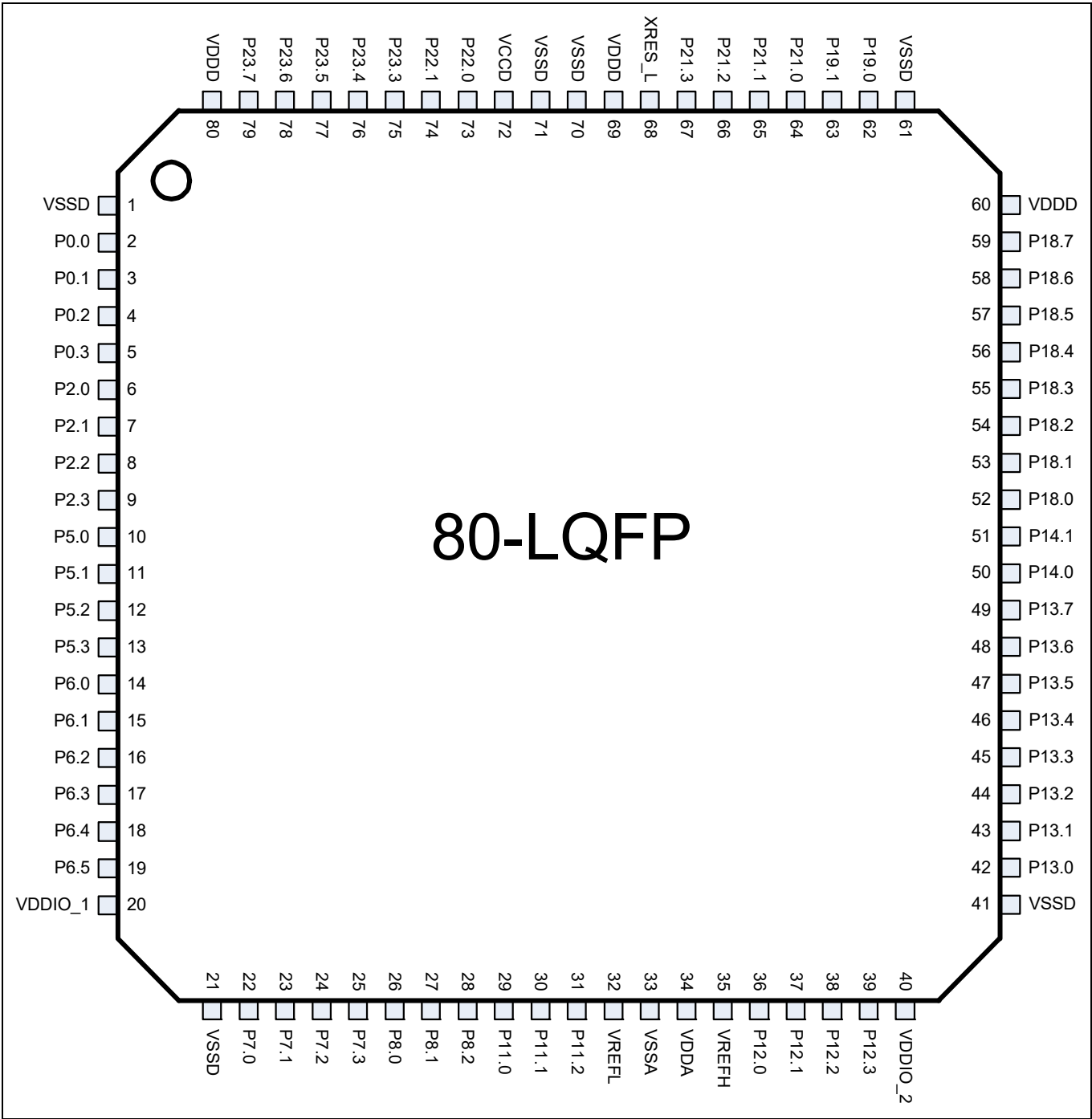
Figure 9-3 80-LQFP pin assignment
