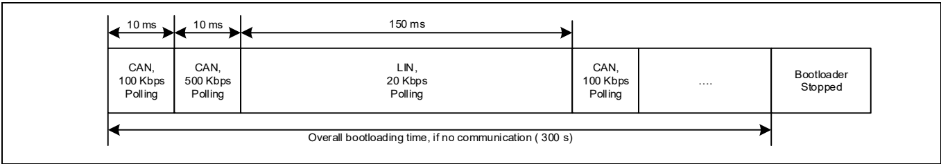
Figure 30-1 Bootloading sequence
