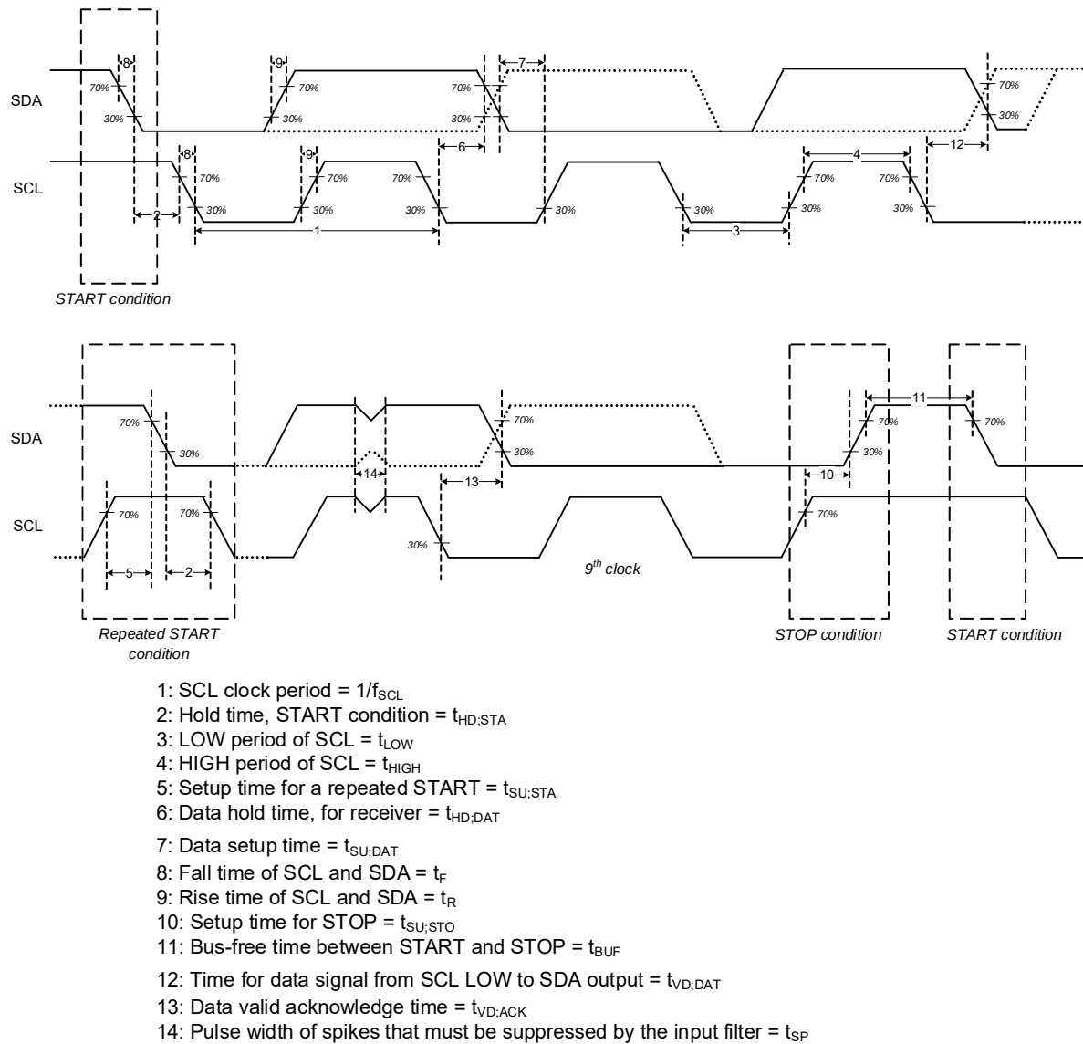
Figure 27-9 I 2 C timing diagrams
