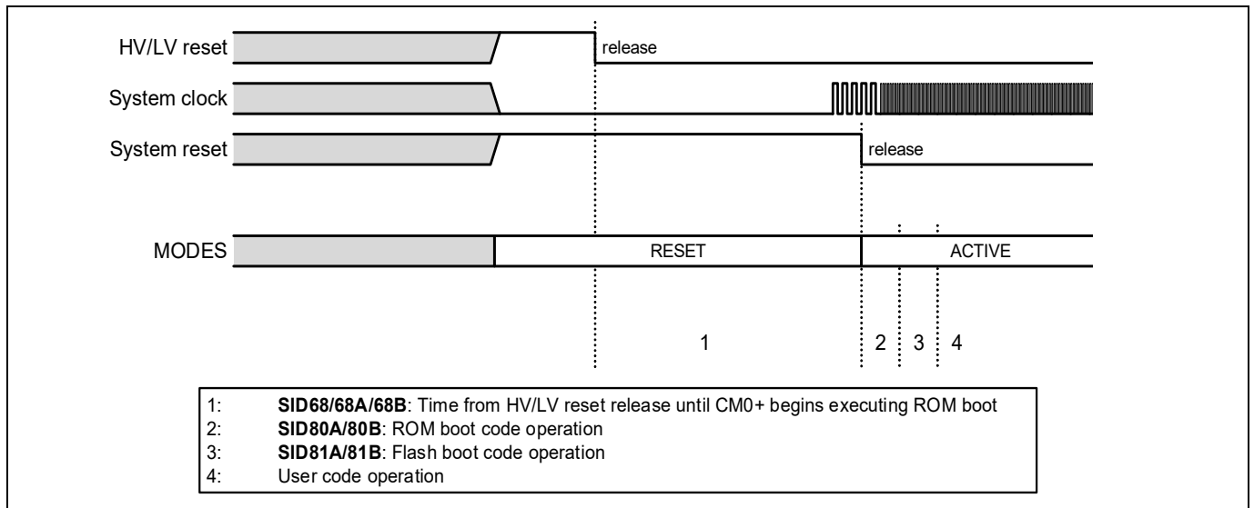
Figure 27-3 Reset sequence
