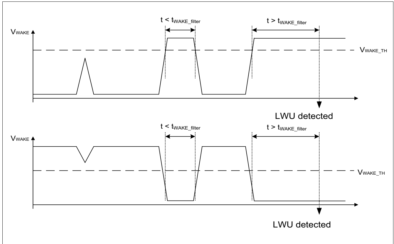
Figure 15 Local Wake-Up
