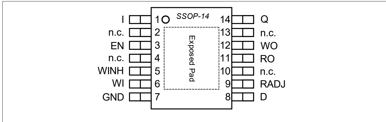
Figure 2 Pin assignment
