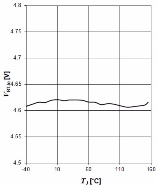
Undervoltage reset lower switching threshold V_{RT,lo} versus junction temperature T_J
