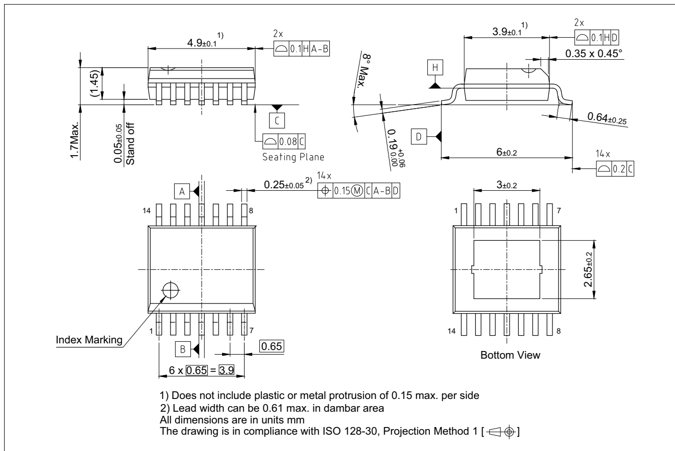
Figure 12 PG-SSOP-14
