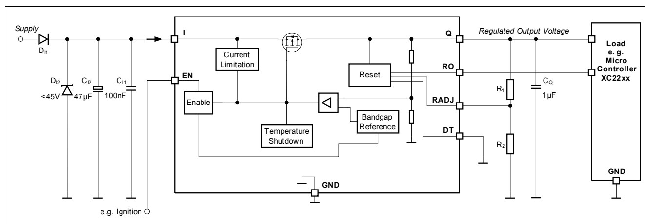
Figure 8 Application Diagram
