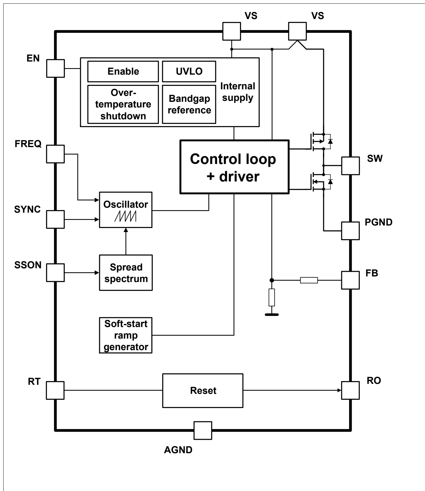
Figure 1 Block diagram
