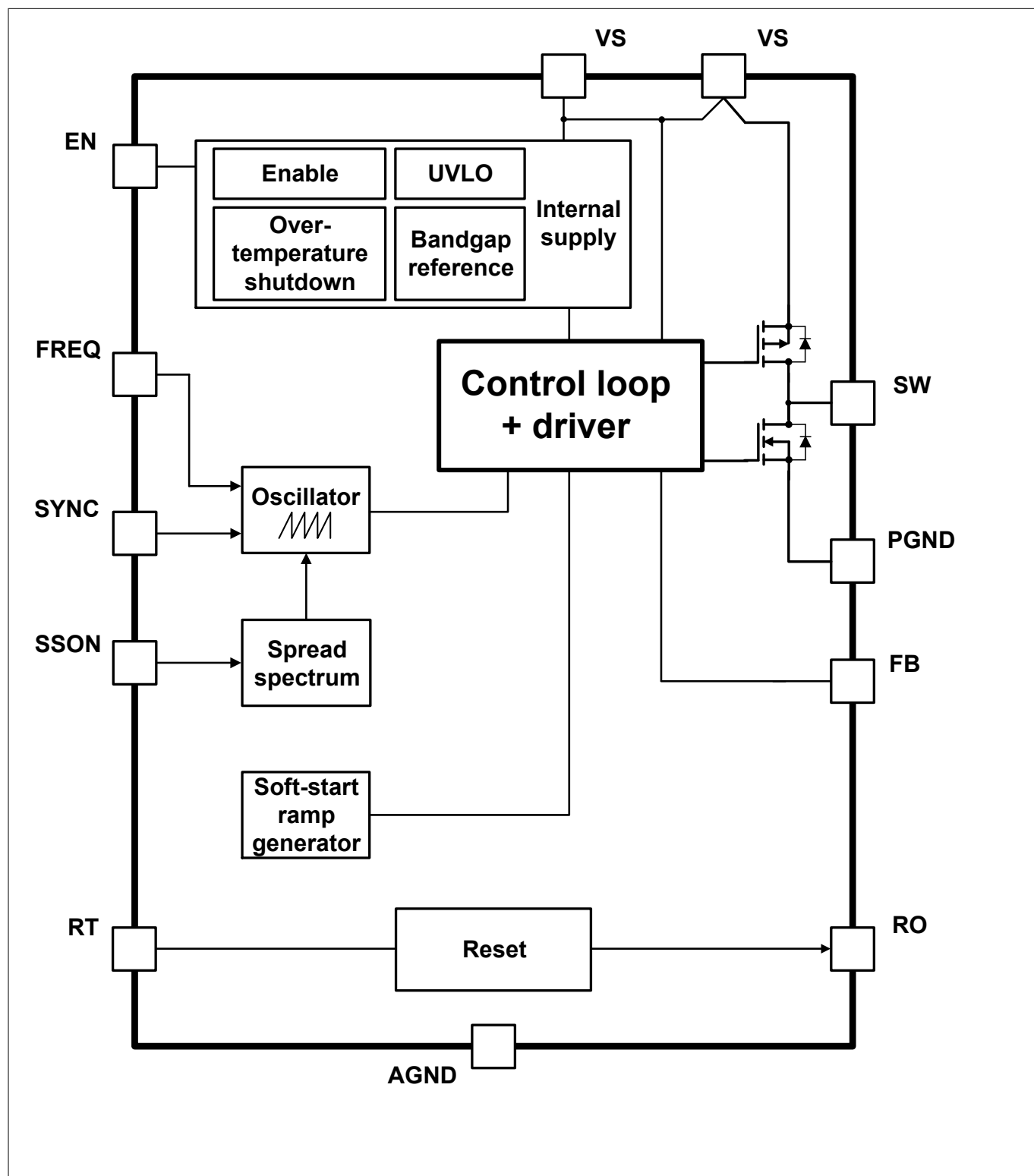
Figure 1 Block diagram
