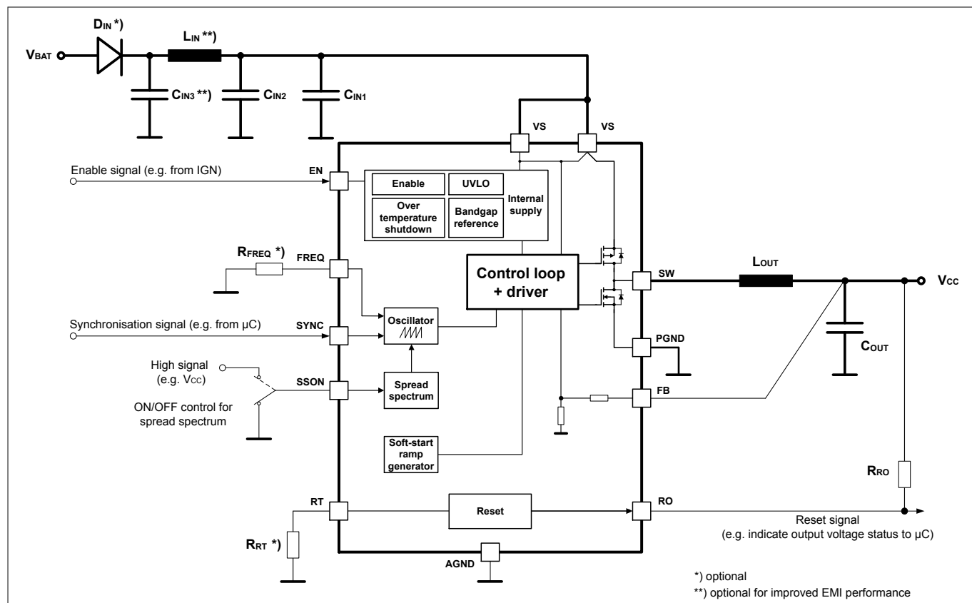
Figure 9 Application diagram
