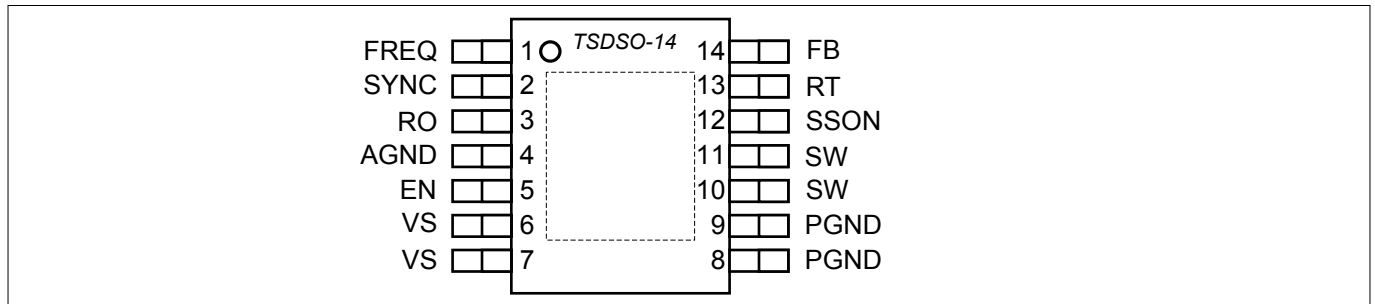
Figure 2 Pin configuration
