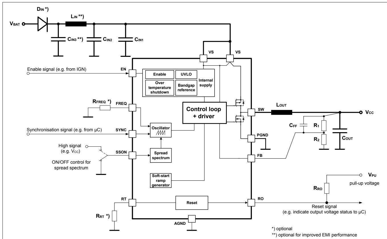
Figure 9 Application diagram
