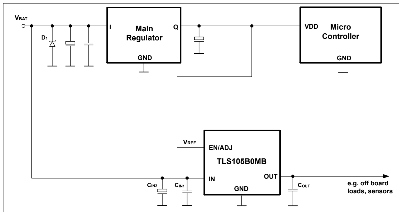
Figure 3 Application circuit
